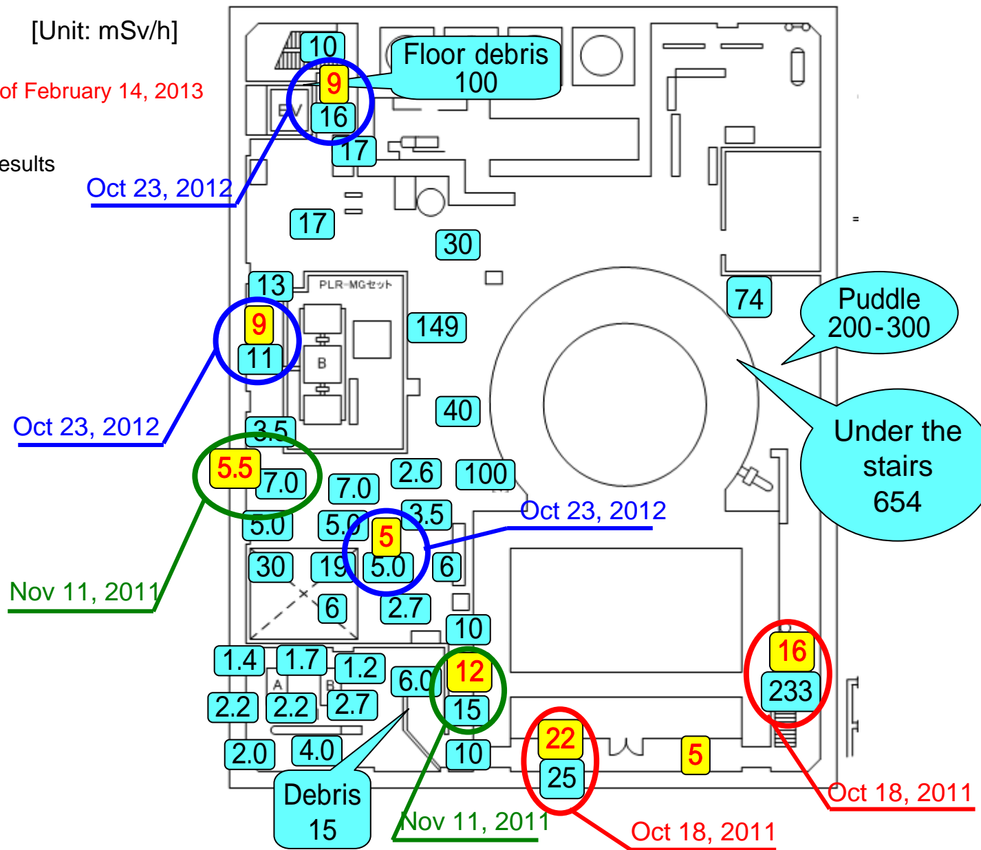
Unit 1 Reactor Building 3F
