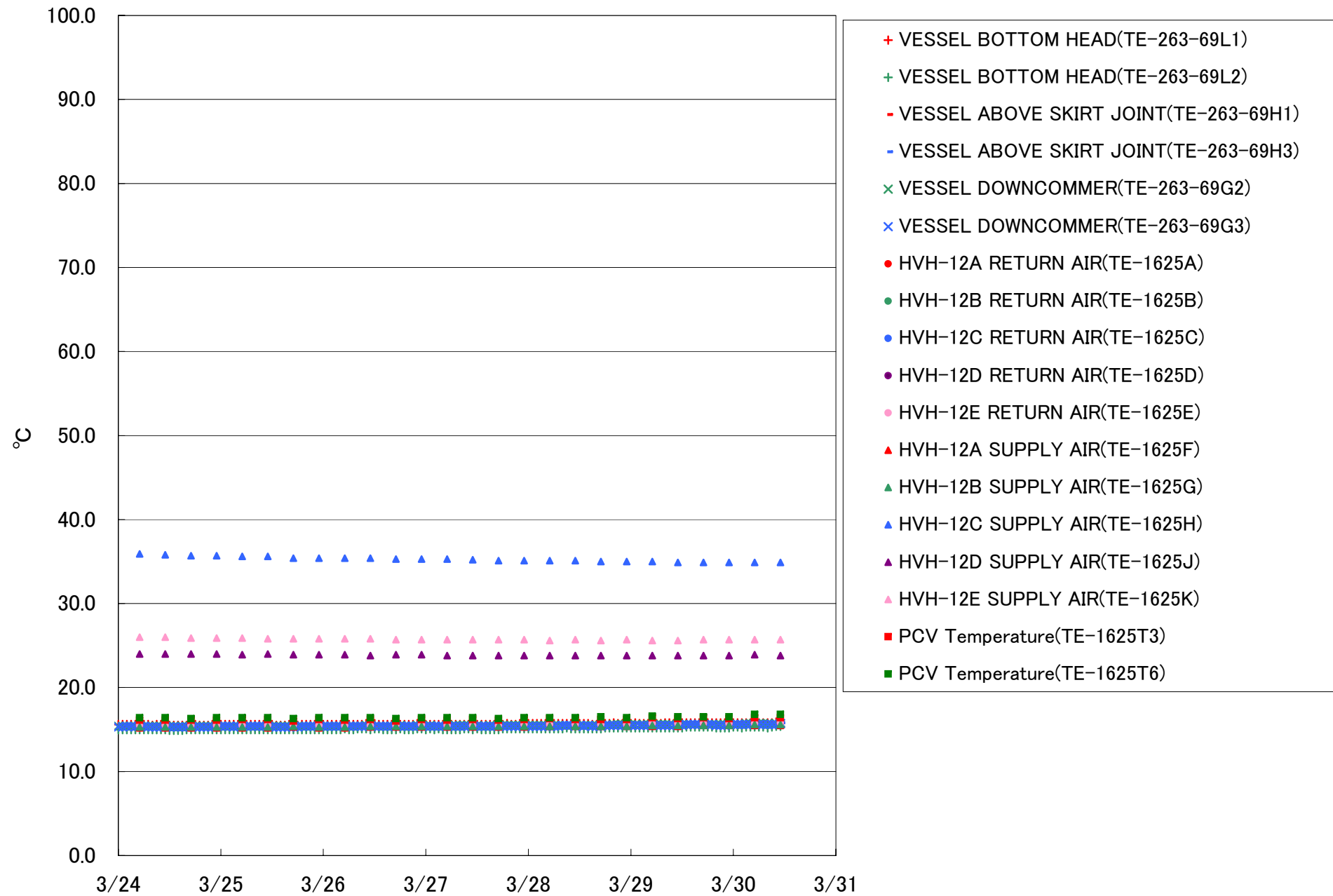
Fukushima Daiichi Nuclear Power Station Unit 1 Parameters of Temperature
