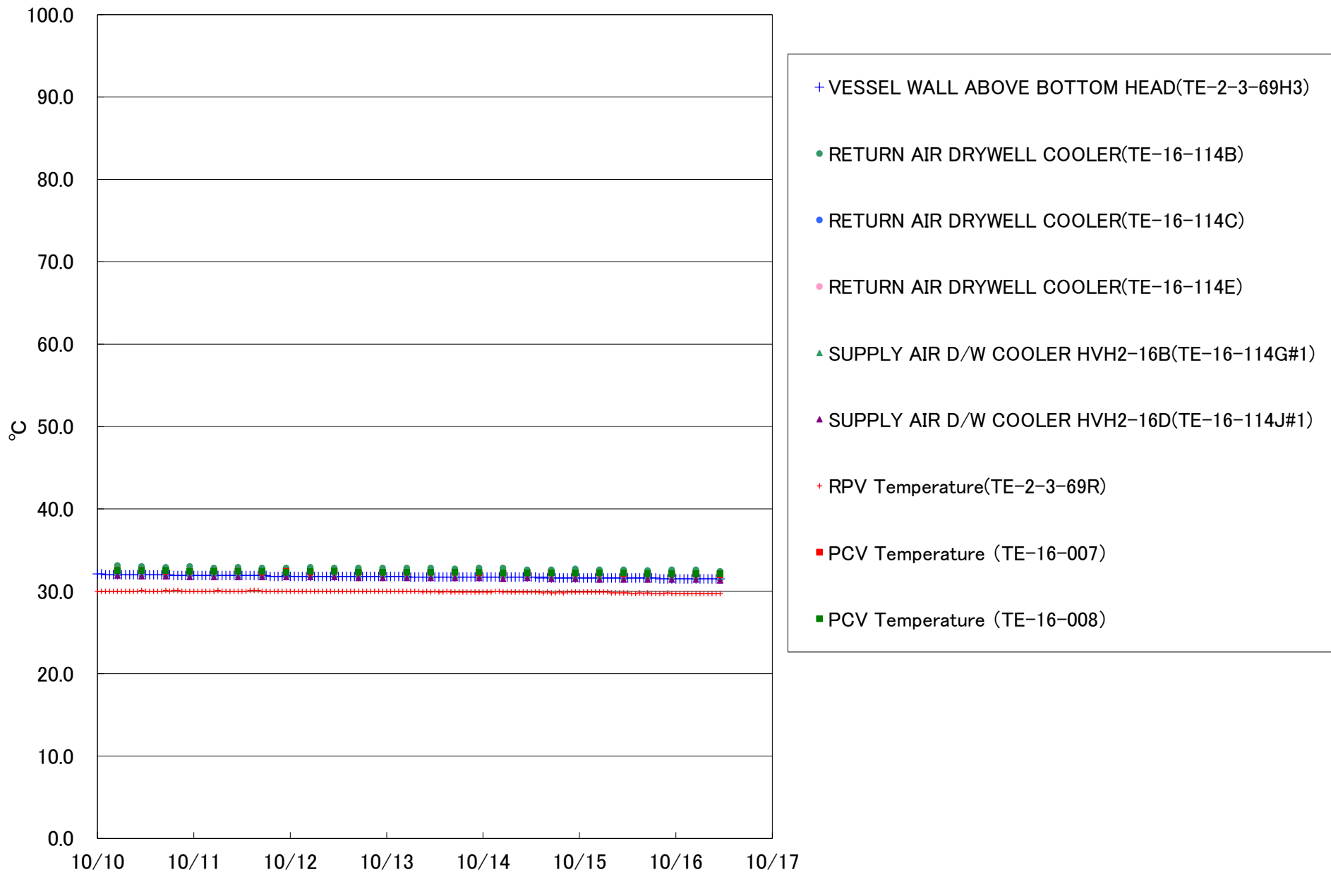
Fukushima Daiichi Nuclear Power Station Unit 2 Parameters of Temperature
