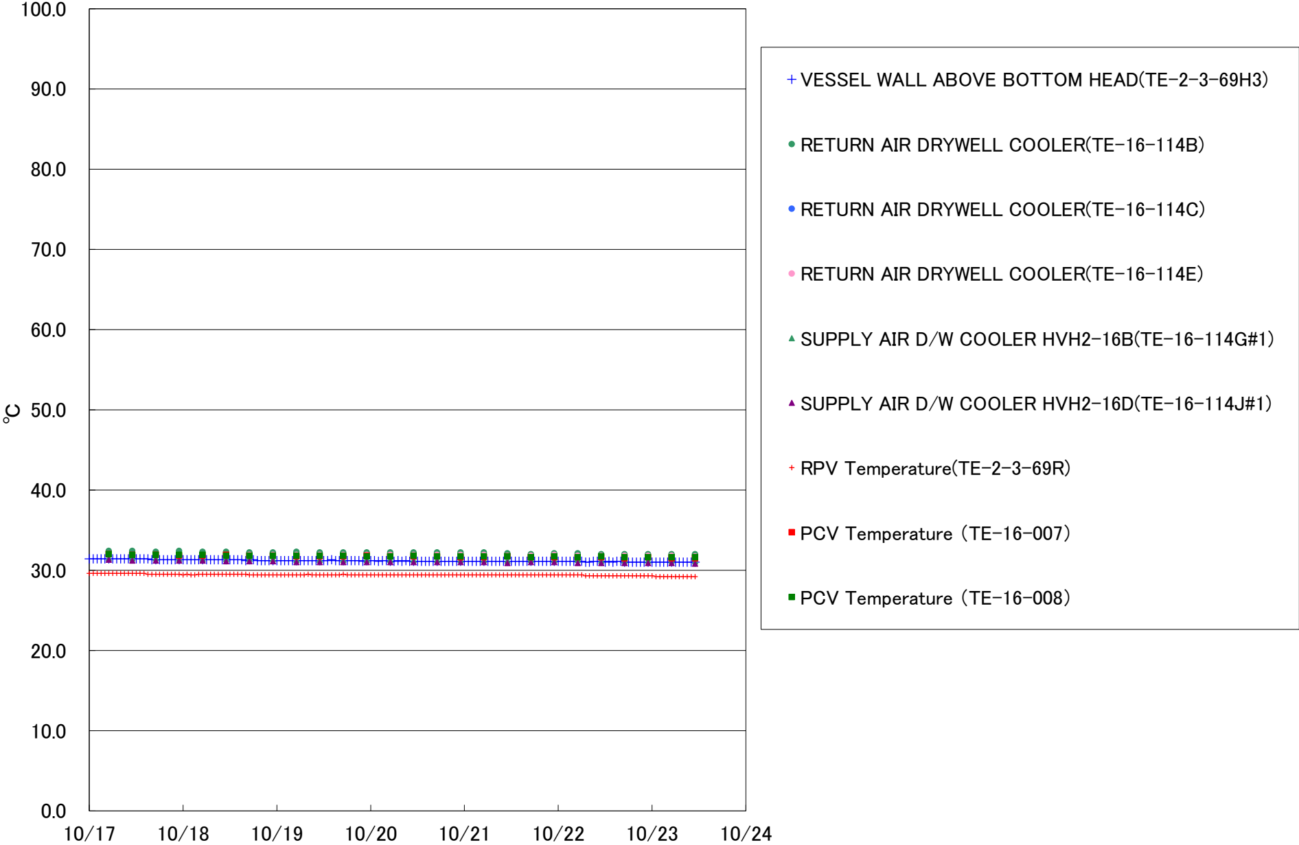
Fukushima Daiichi Nuclear Power Station Unit 2 Parameters of Temperature
