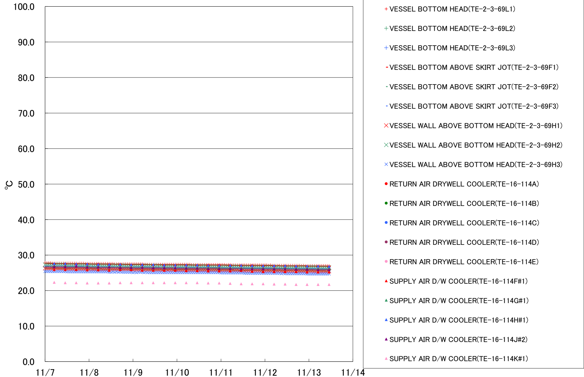
Fukushima Daiichi Nuclear Power Station Unit 3 Parameters of Temperature
