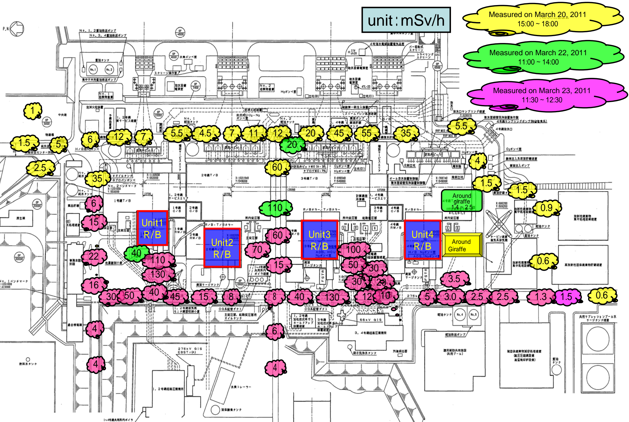
Around concrete pumping vehicle called "Giraffe"
