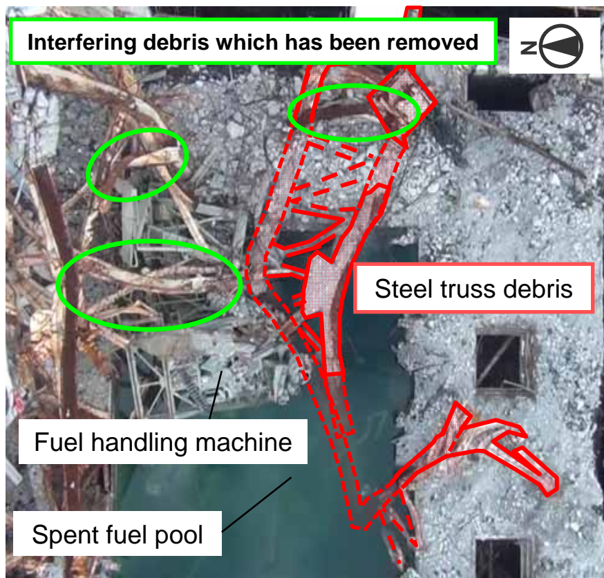
Interfering debris (Before removal)
