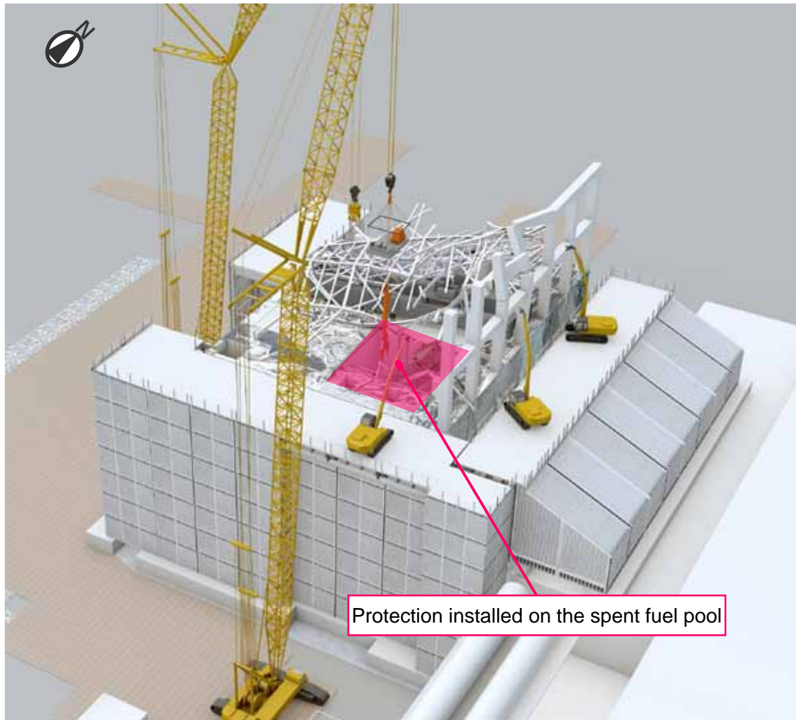
Debris removal from the upper part of the operation floor
