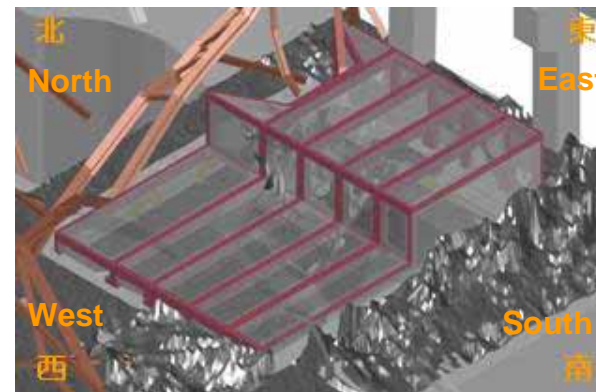
Protection installed on the spent fuel pool
