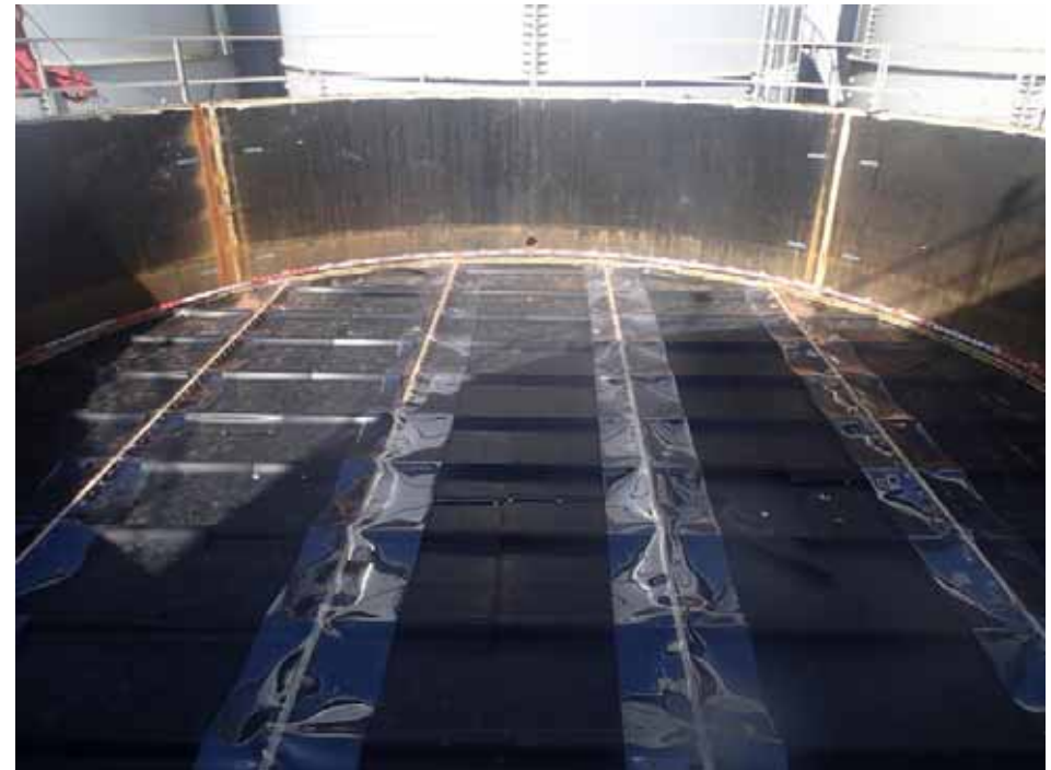
The tank No.5 in H4 area The bottom plates (with protection materials) (Photo taken on September 19, 2013)
