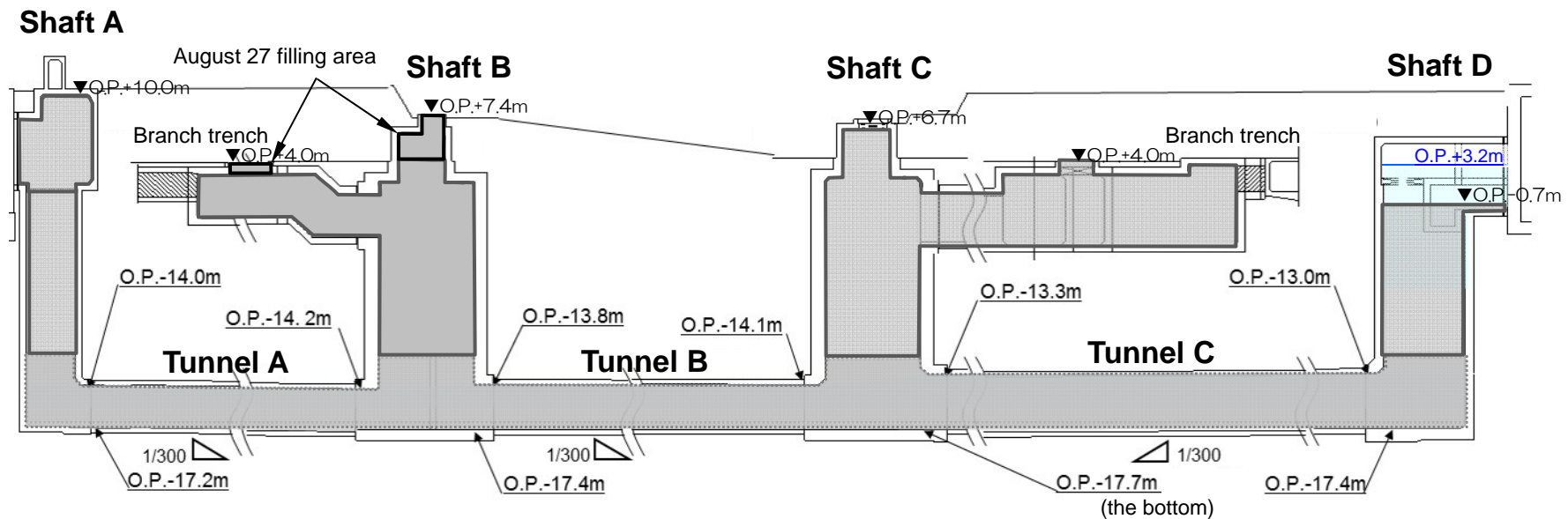
Unit 3 Seawater piping trench schematic cross-sectioned view
