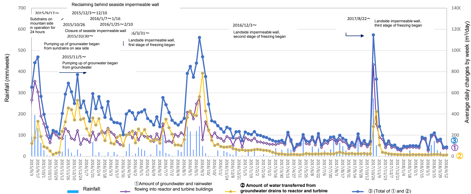
Amount of water transferred from groundwater drains to reactor and turbine buildings (From April 5, 2018 to April 11, 2018)
