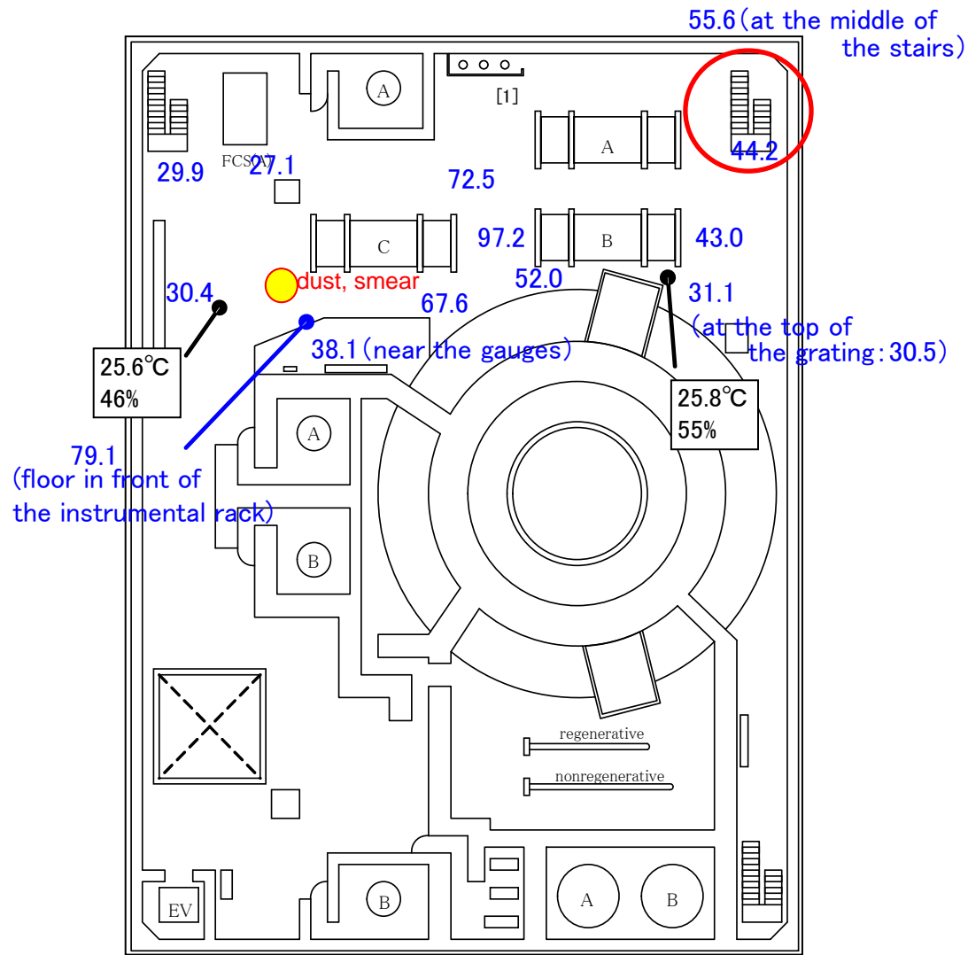
2nd floor of the reactor building
