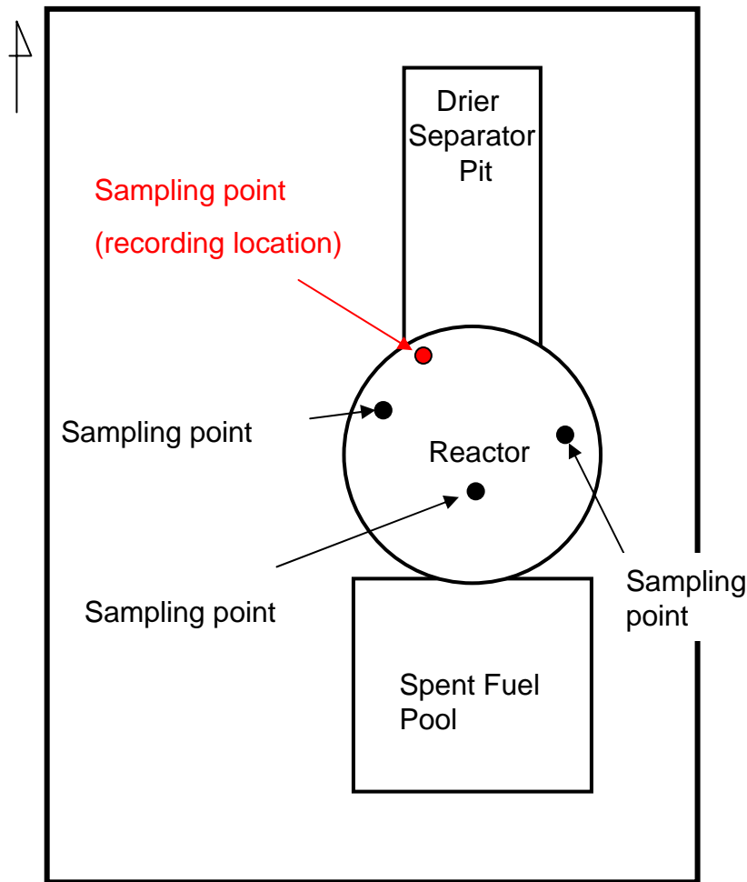
Layout drawing of 5 th floor of Unit 3 reactor building in Fukushima Daiichi Nuclear Power Station
