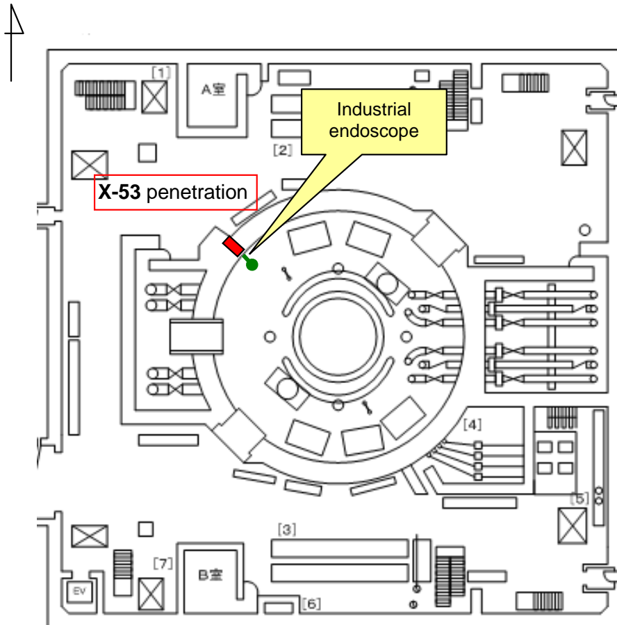
Layout drawing of 1st floor of Unit 5 reactor building in Fukushima Daiichi Nuclear Power Station
