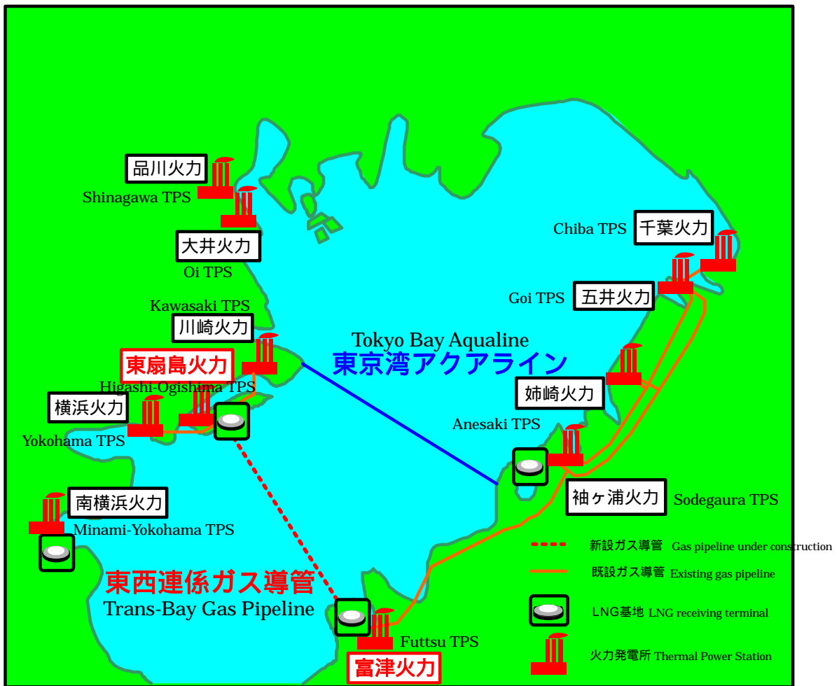
Map of TEPCO gas pipelines and the Trans-Bay Gas Pipeline
