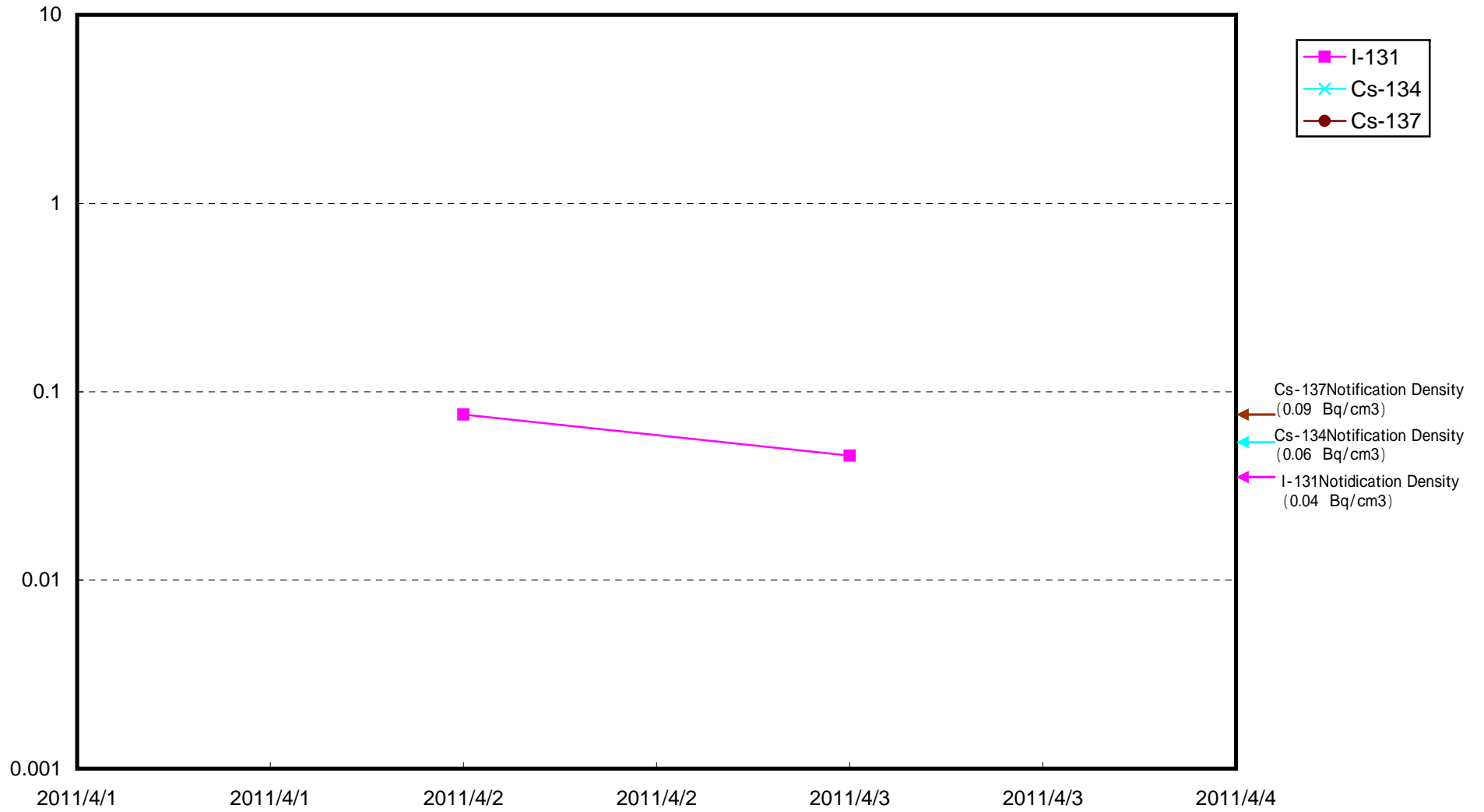
Radioactivity Density at 15km off shore Iwasawa Shore (Bq/cm3)
