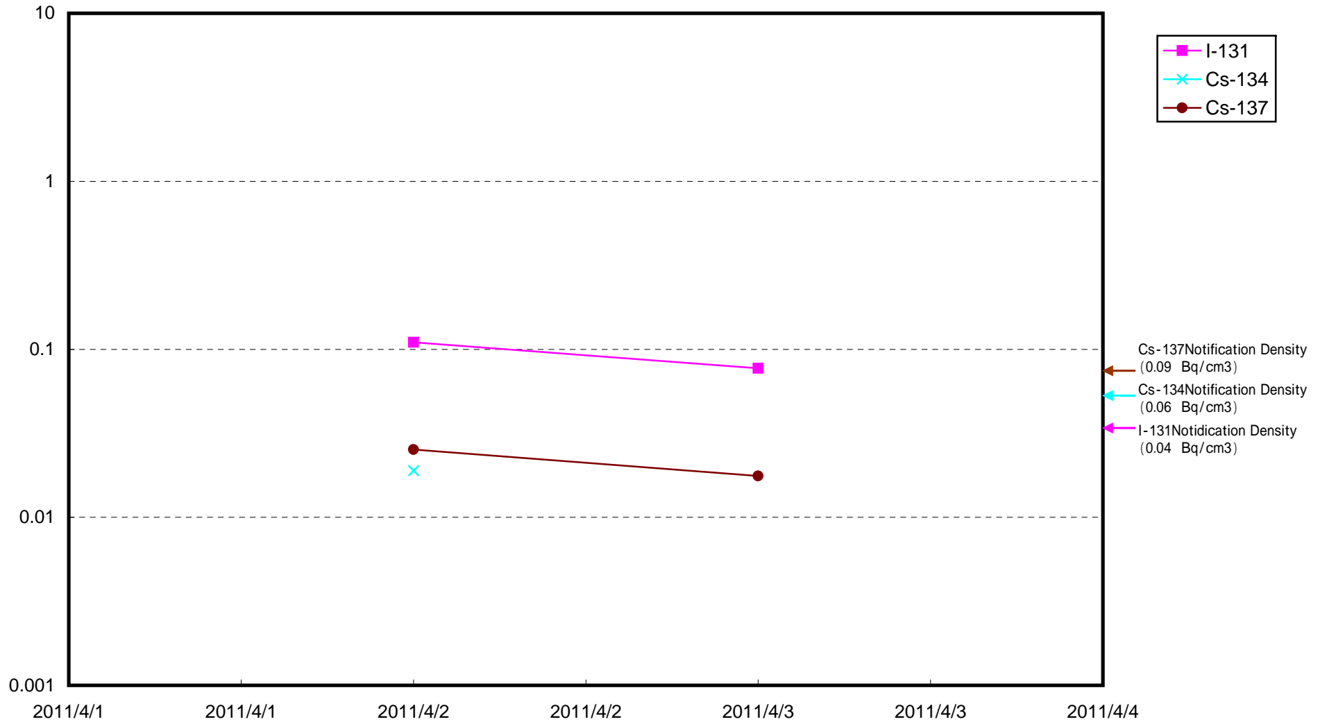
Radioactivity Density at 15km off shore 2F NPS (Bq/cm3)
