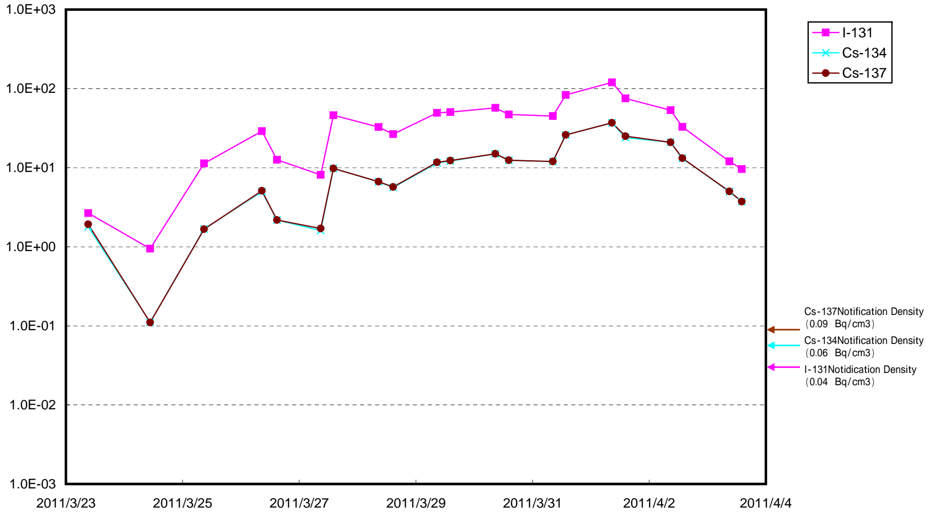
Radioactivity Density at 1F 5 ~ 6 Discharge Canal (North) (approx. 30km north of 5 ~ 6u discharge canal) (Bq/cm 3 )
