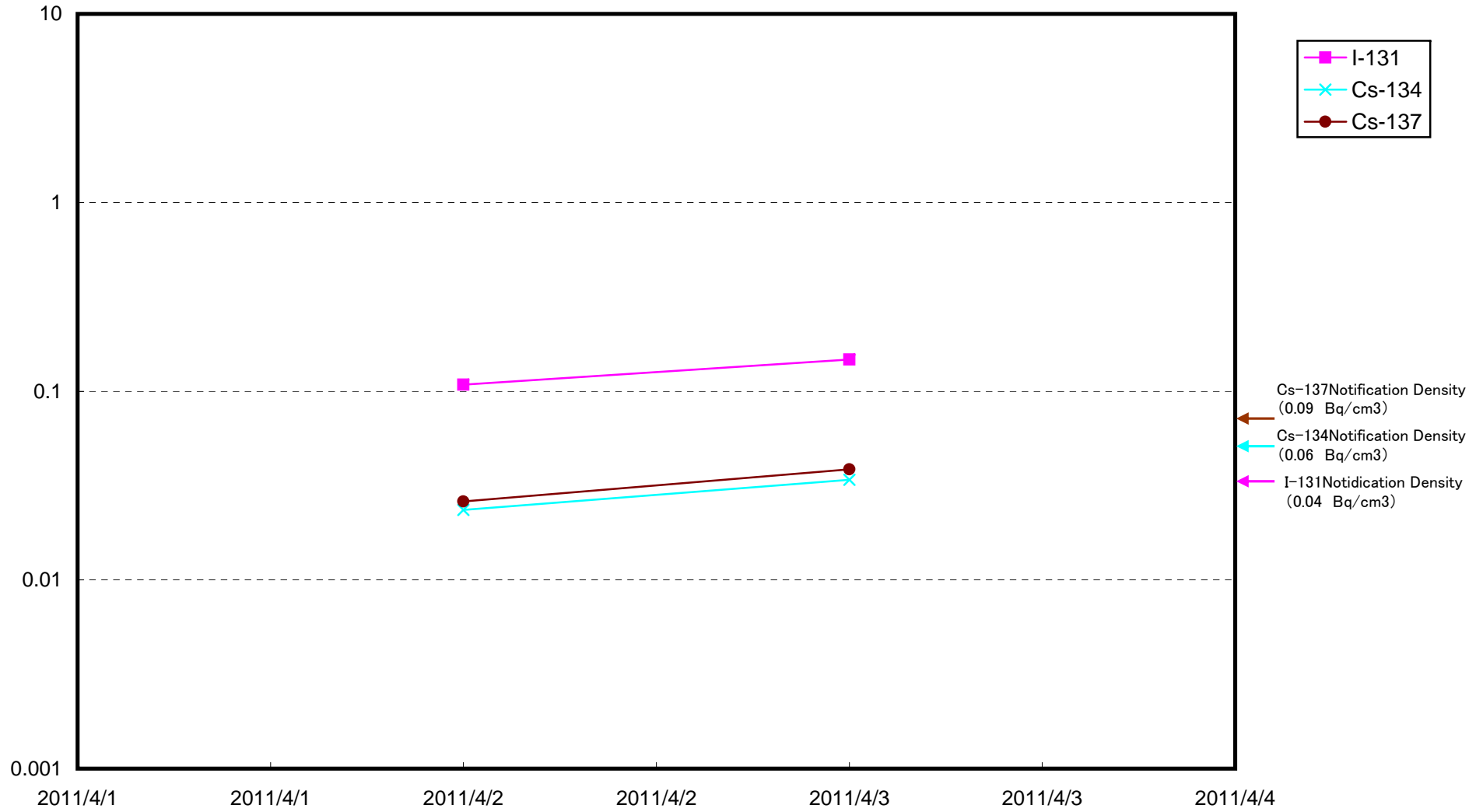
Radioactivity Density at 15km off shore 1F NPS (Bq/cm3)
