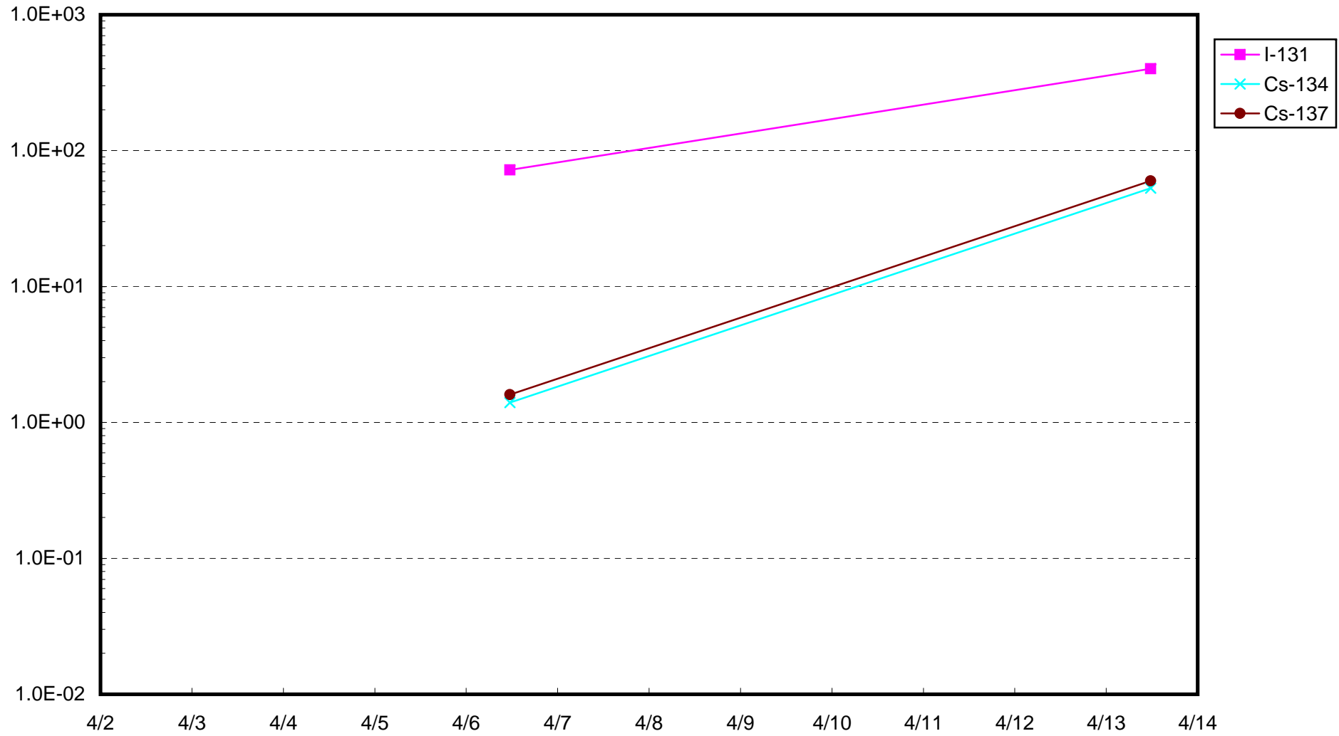
Fukushima Daiich Nuclear Power Station : Radioactivity Density of Sub-drain of Unit 1 ( B q / c m 3 )
