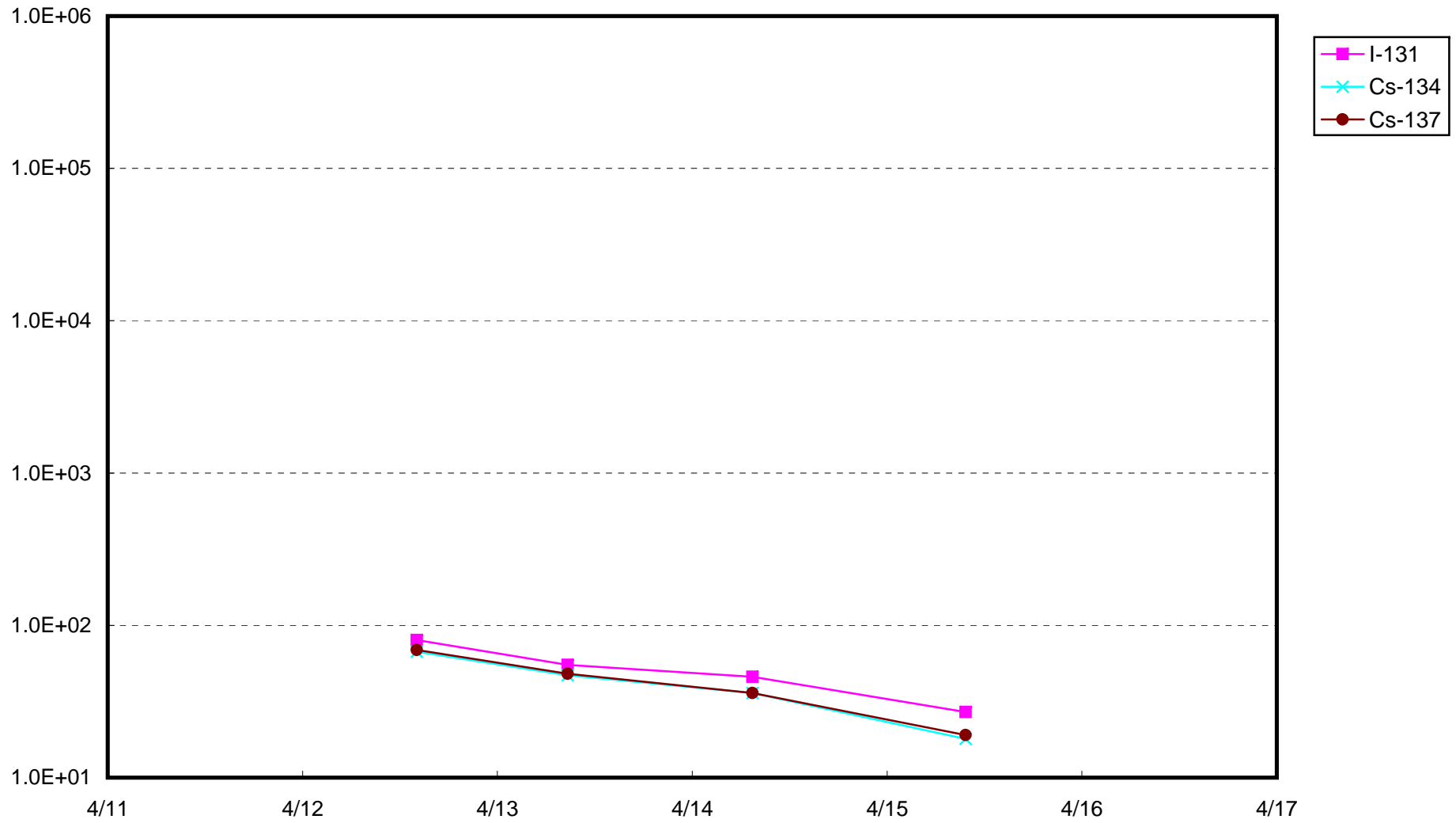
Radioactivity density of seawater at the north of Unit 1 - 4 water intake, Fukushima Daiichi NPS (Bq/cm 3 )
