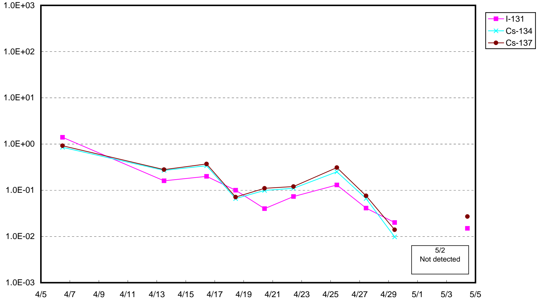
Fukushima Daiichi Nuclear Power Station : Radioactivity Density at Sub-drain of Unit 5 ( B q / c m 3 )
