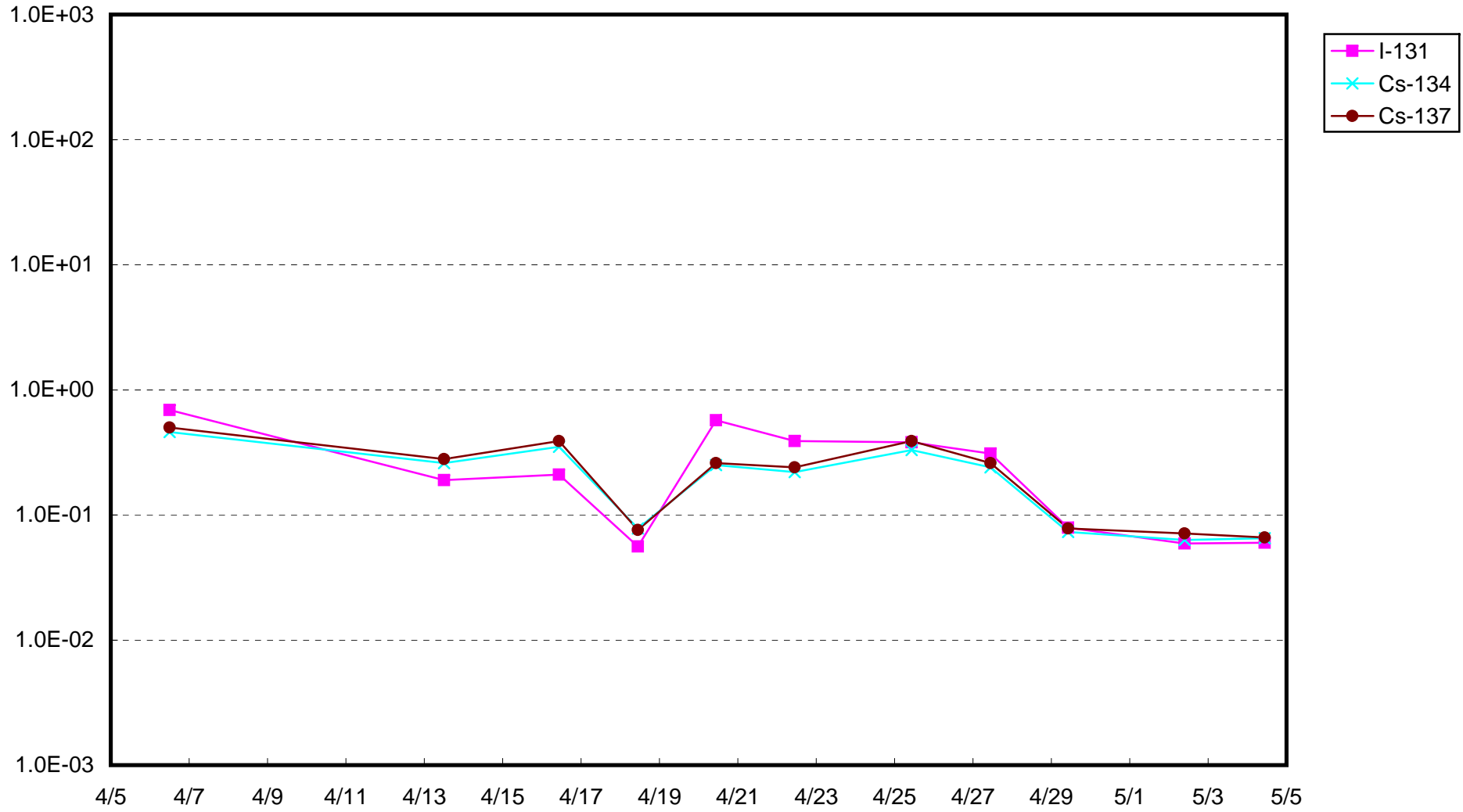
Fukushima Daiichi Nuclear Power Station : Radioactivity Density at Sub-drain of Unit 6 ( B q / c m 3 )
