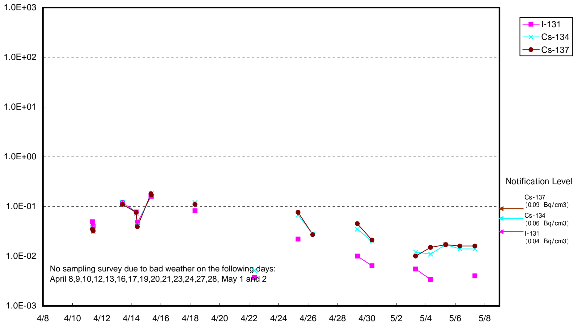
Radioactivity Density of Seawater around approx. 15 km offshore of Iwasawa Shore (Bq/cm 3 )
