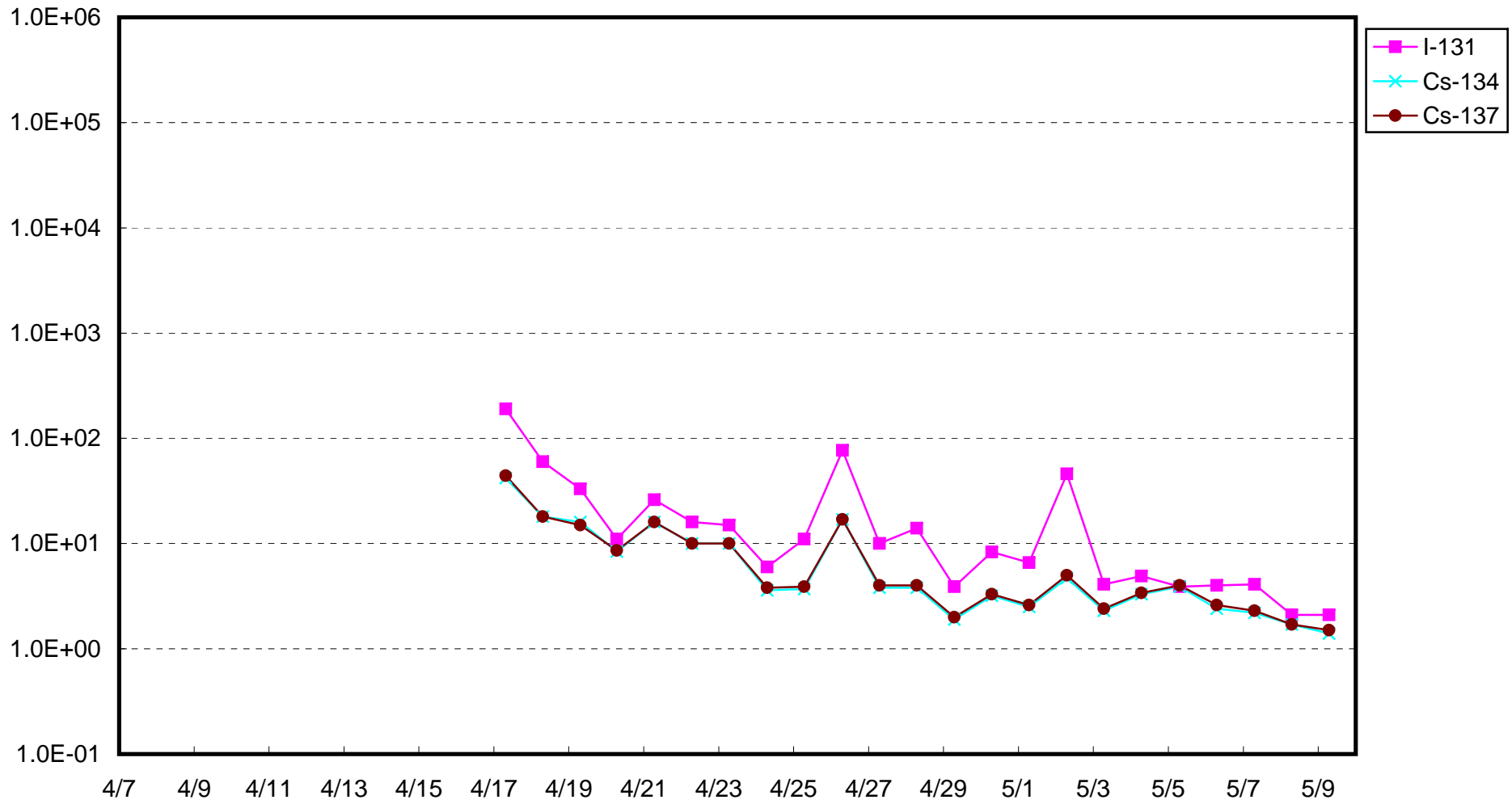
Radioactivity density of Seawater around the Bar Screen of Unit 2 of Fukushima Daiichi NPS (outside of the Silt Fence) (Bq/cm 3 )
