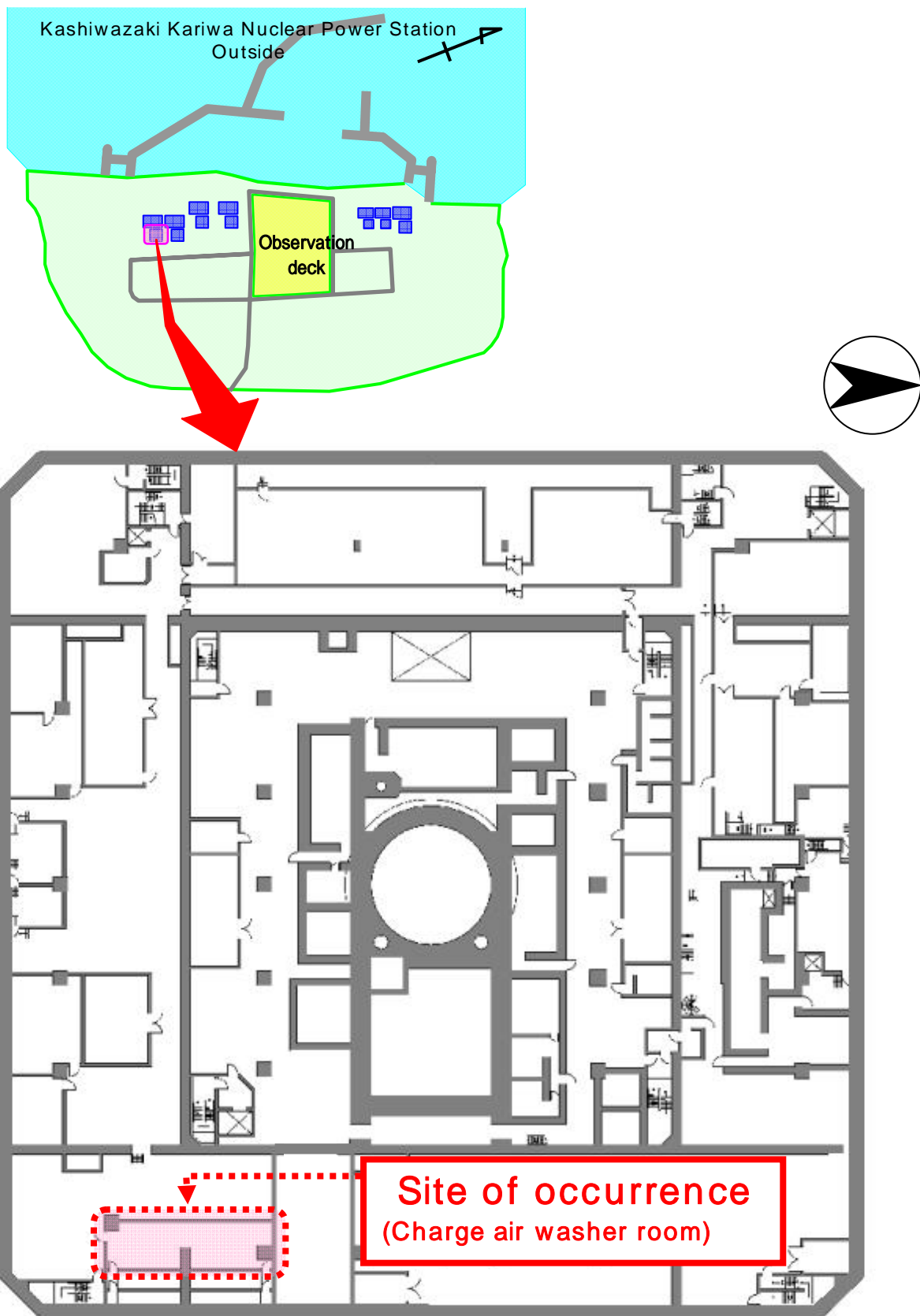
Kashiwazaki Kariwa Nuclear Power Station Unit 1 Reactor building 1st Floor
