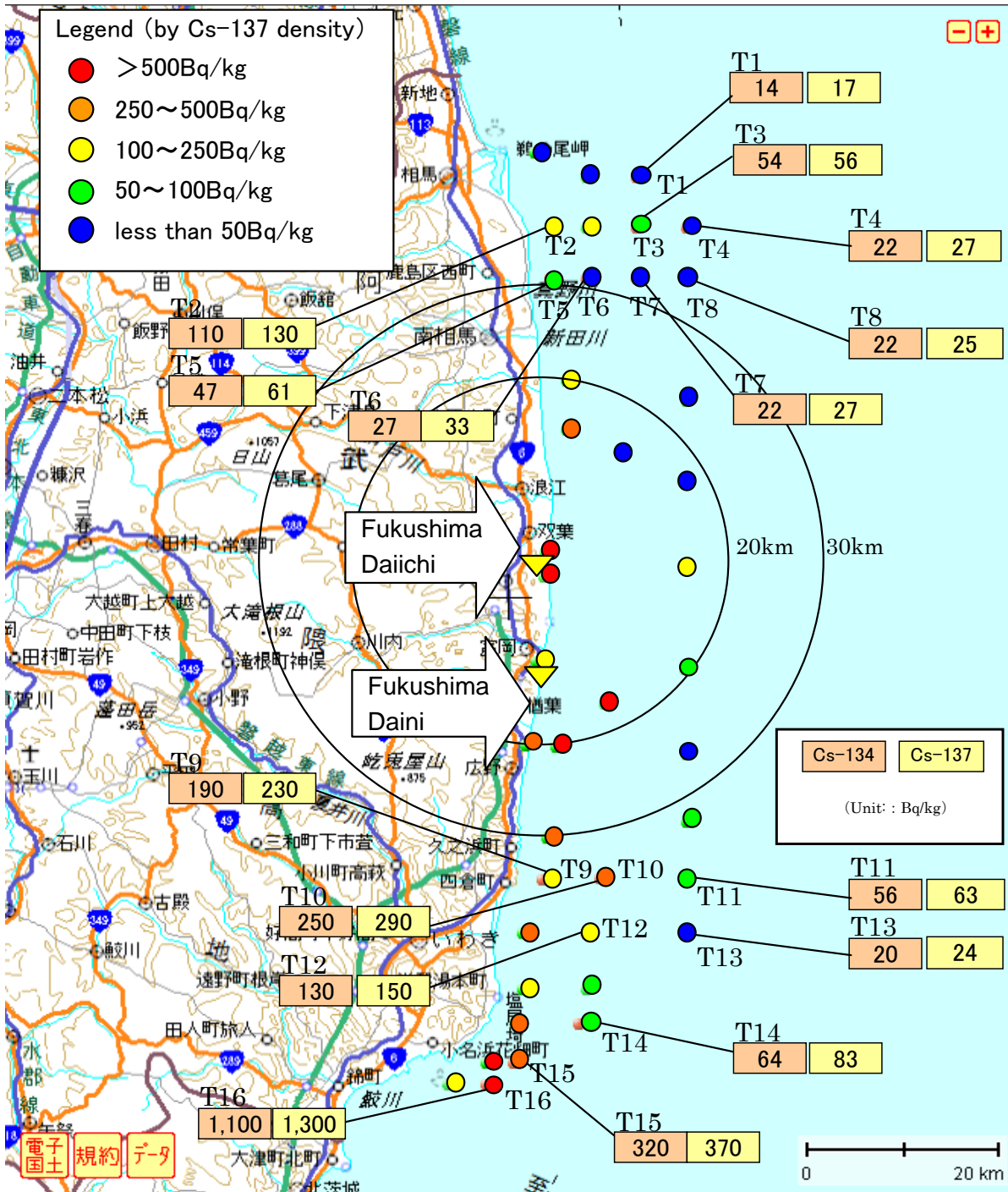
Readings of Additional Sea Area Monitoring at offshore of Fukushima Prefecture -marine soil- (September 26– 28,2011)
