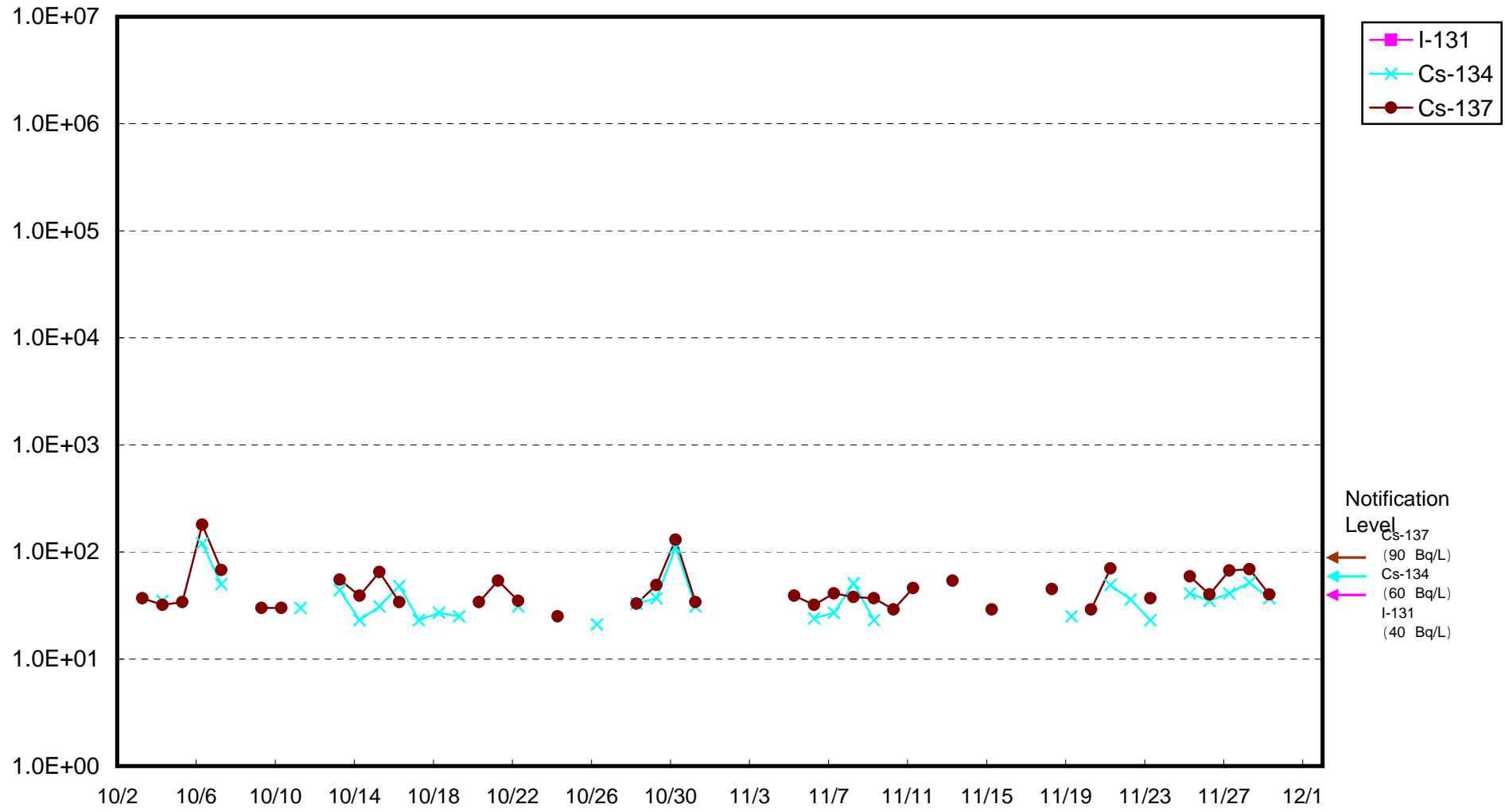
Radioactivity Density of Seawater in front of Shallow Draft Quay of 1F (Bq/L)
