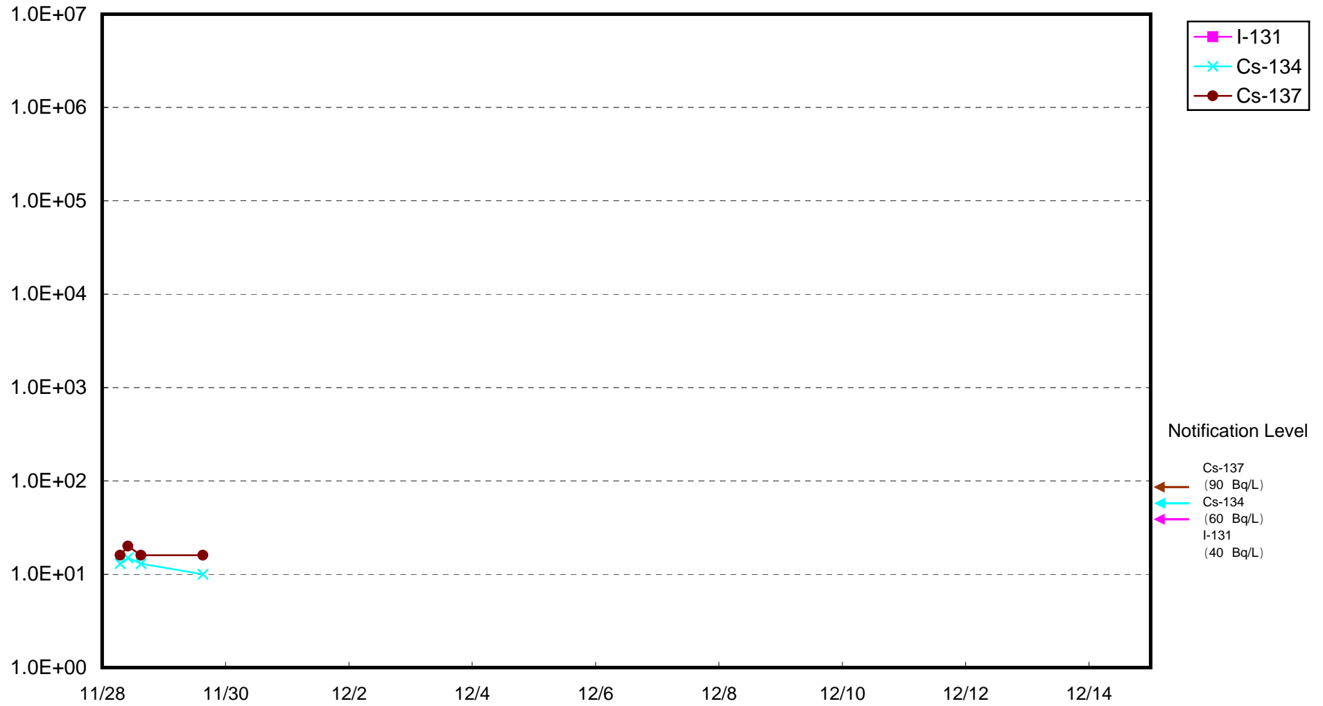
Radioactivity density of seawater near the intake of Fukushima Daiichi Unit 5 ( B q / L )
