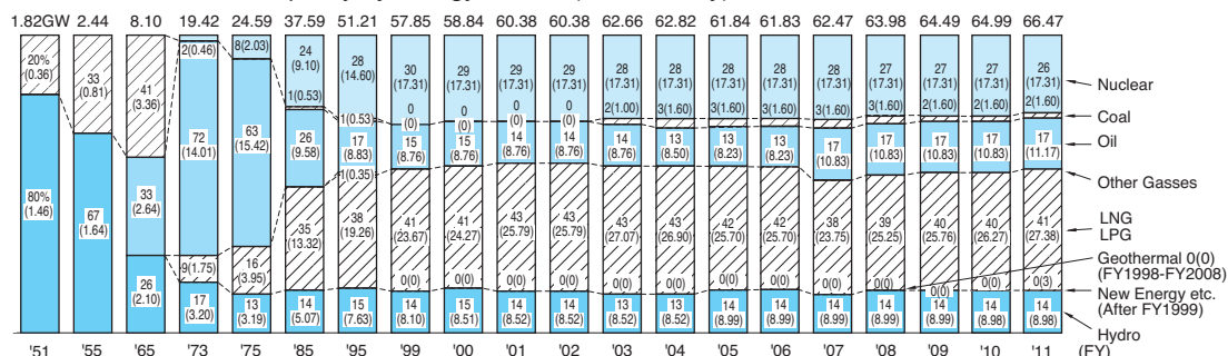
a. Generation Capacity by Energy Source (TEPCO only)
