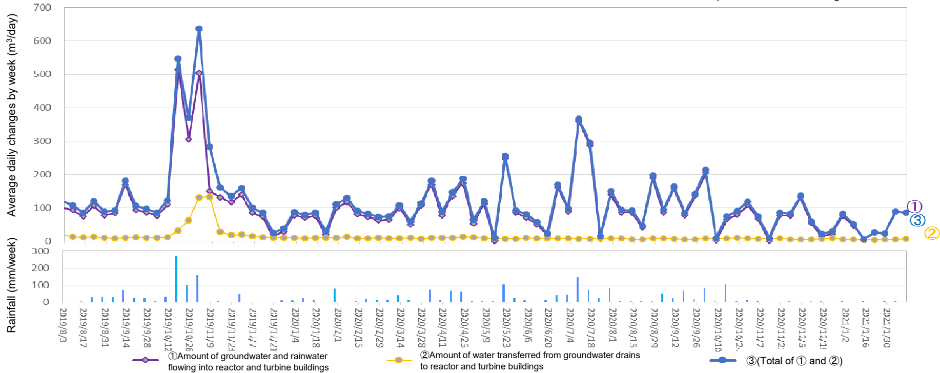
Amount of water transferred from groundwater drains to reactor and turbine buildings (From Feb 4, 2021 to Feb 10, 2021)
