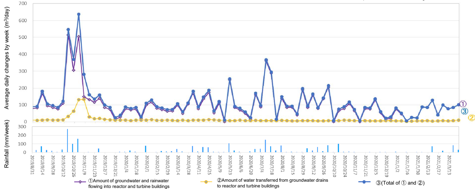
Amount of water transferred from groundwater drains to reactor and turbine buildings (From Mar 18, 2021 to Mar 24, 2021)
