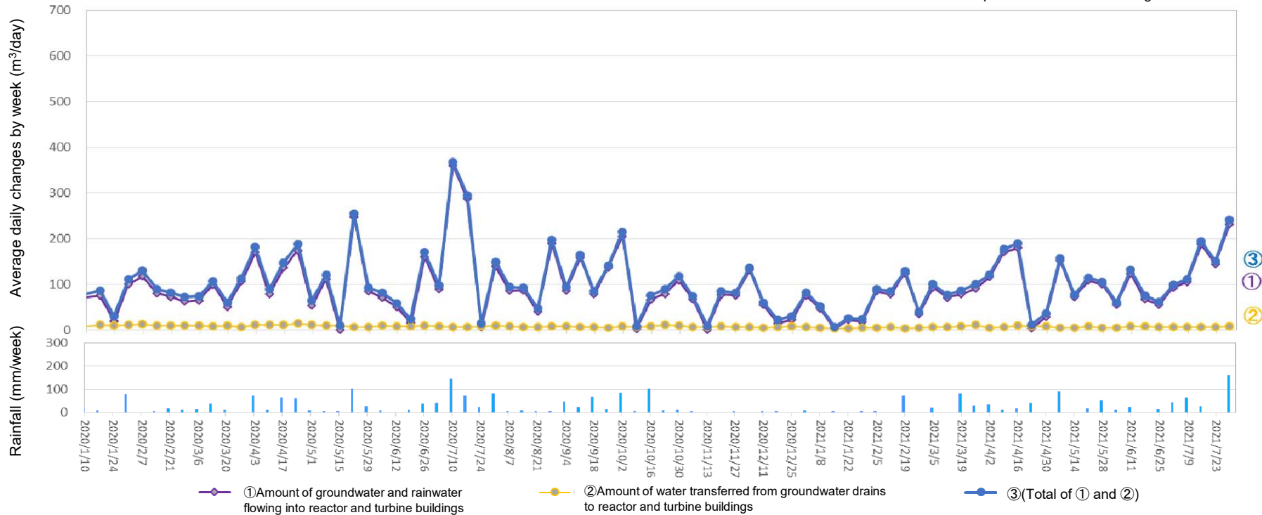
Amount of water transferred from groundwater drains to reactor and turbine buildings (From July 22, 2021 to July 28, 2021)
