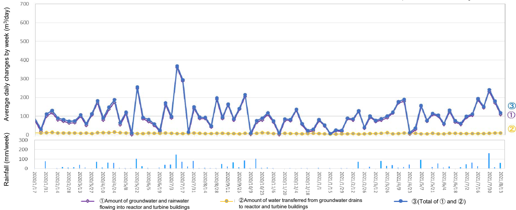
Amount of water transferred from groundwater drains to reactor and turbine buildings (From August 5, 2021 to August 11, 2021)
