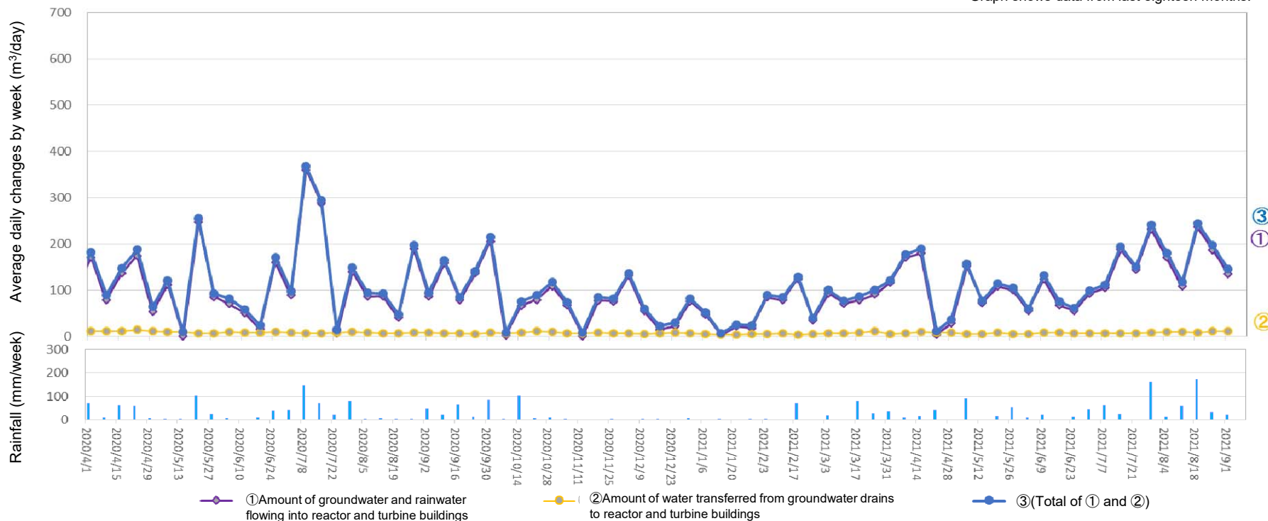
Amount of water transferred from groundwater drains to reactor and turbine buildings (From August 26, 2021 to September 1, 2021)
