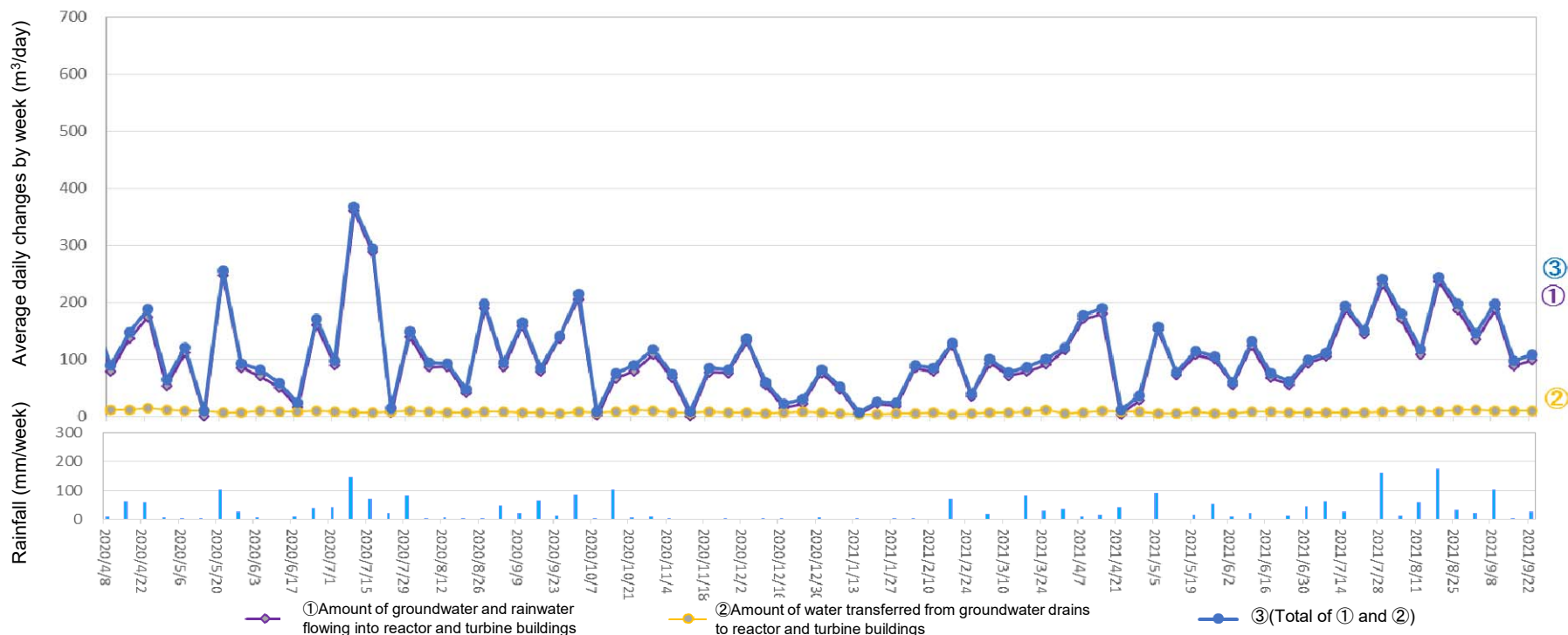
Amount of water transferred from groundwater drains to reactor and turbine buildings (From September 16, 2021 to September 22, 2021)
