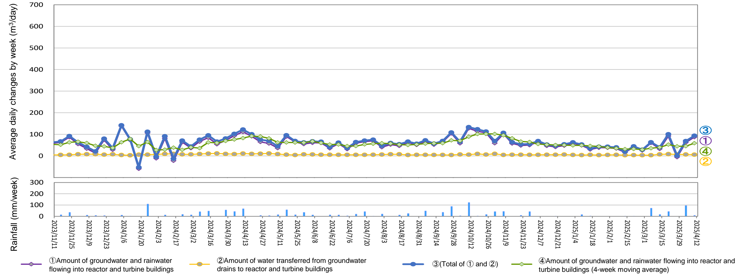
Amount of water transferred from groundwater drains to reactor and turbine buildings (From Apr 3, 2025 to Apr 9, 2025)
