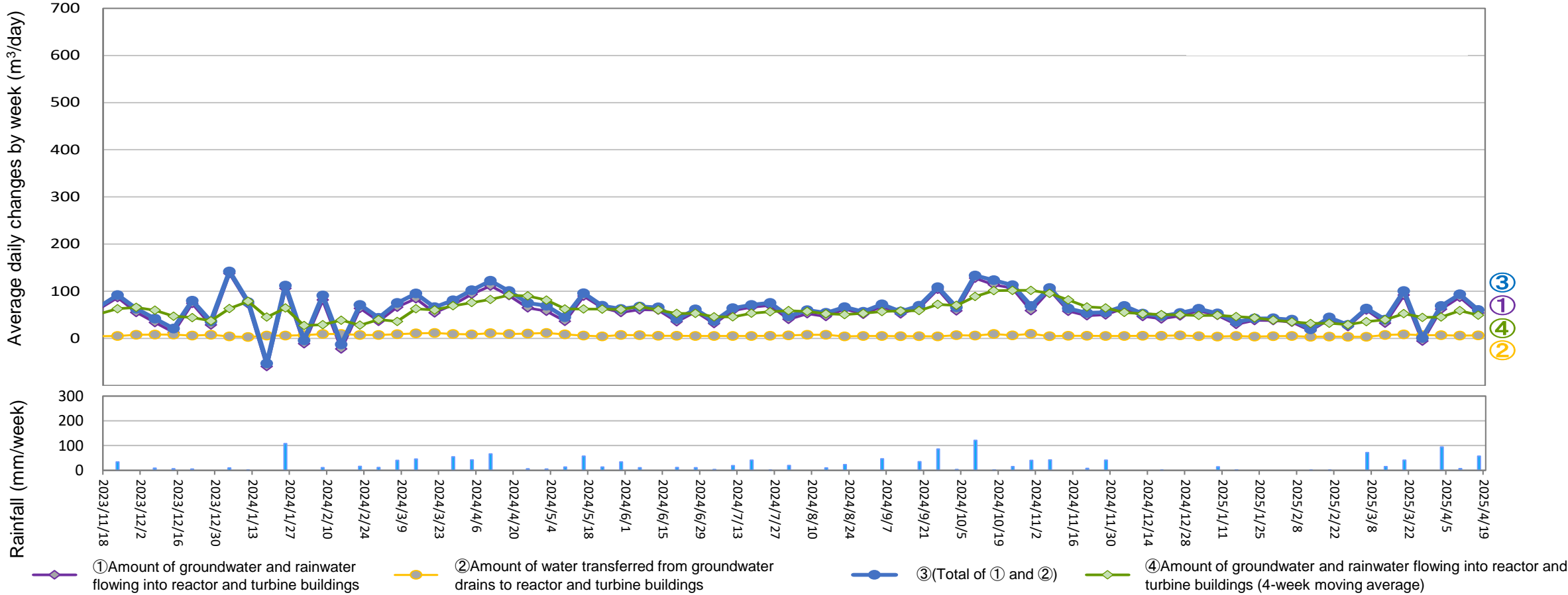
Amount of water transferred from groundwater drains to reactor and turbine buildings (From Apr 10, 2025 to Apr 16, 2025)
