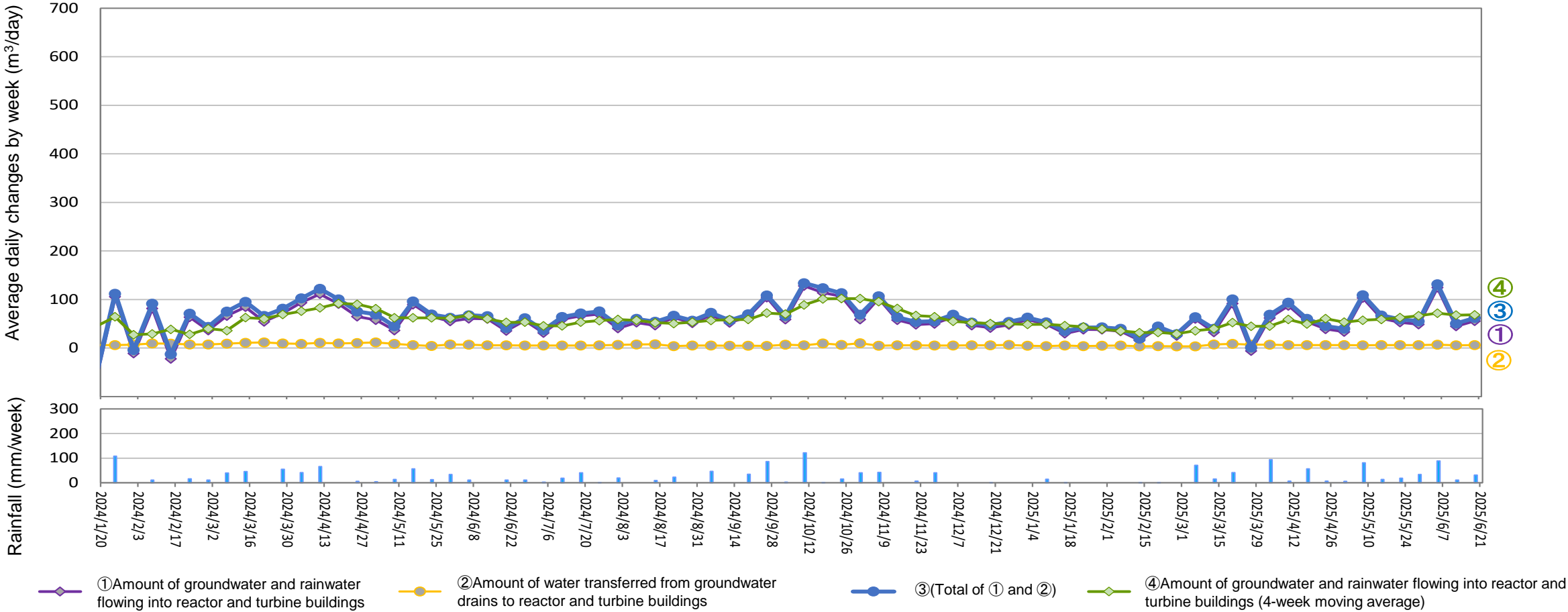
Amount of water transferred from groundwater drains to reactor and turbine buildings (From June 12, 2025 to June 18, 2025)
