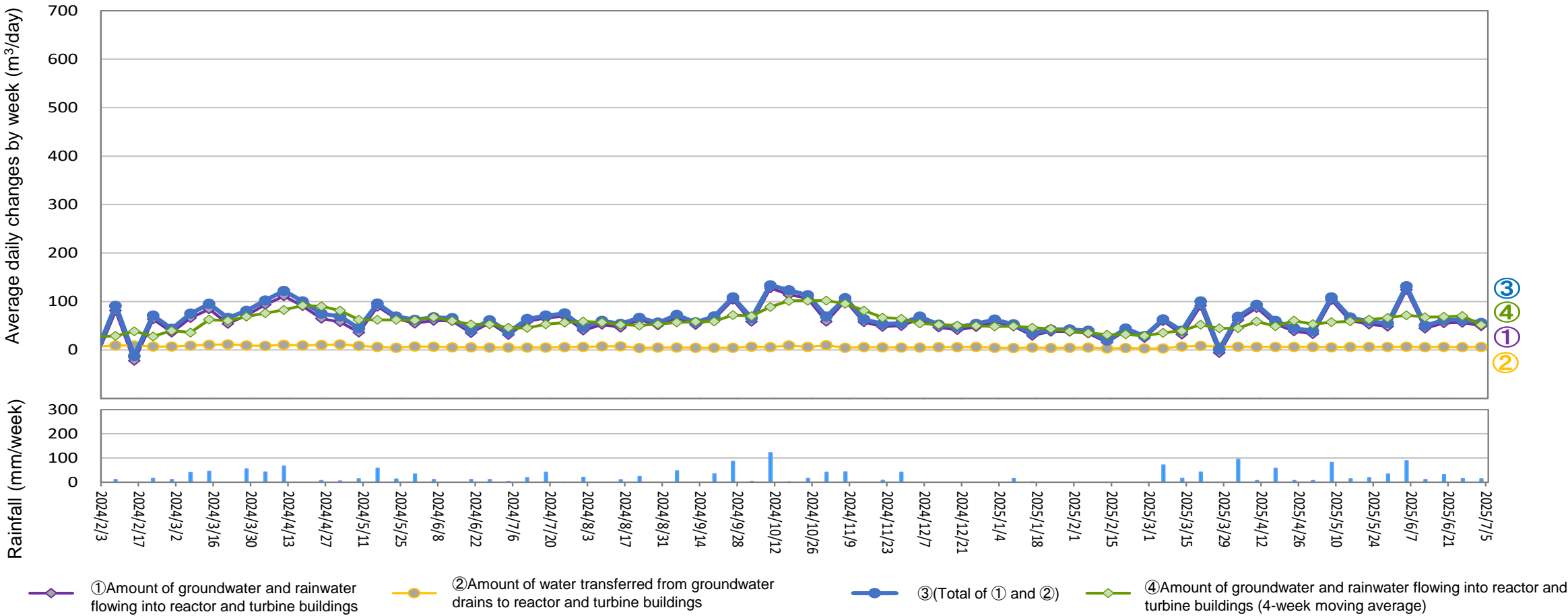
Amount of water transferred from groundwater drains to reactor and turbine buildings (From June 26, 2025 to July 2, 2025)
