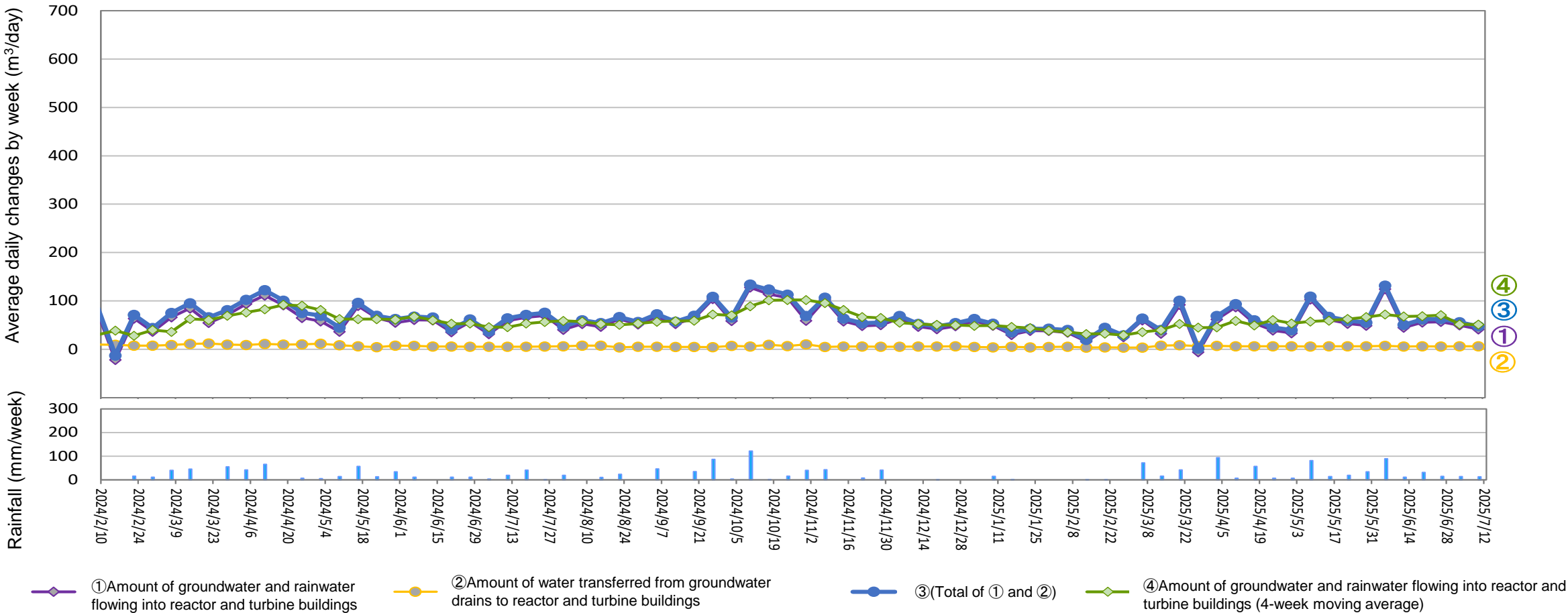
Amount of water transferred from groundwater drains to reactor and turbine buildings (From July 3, 2025 to July 9, 2025)
