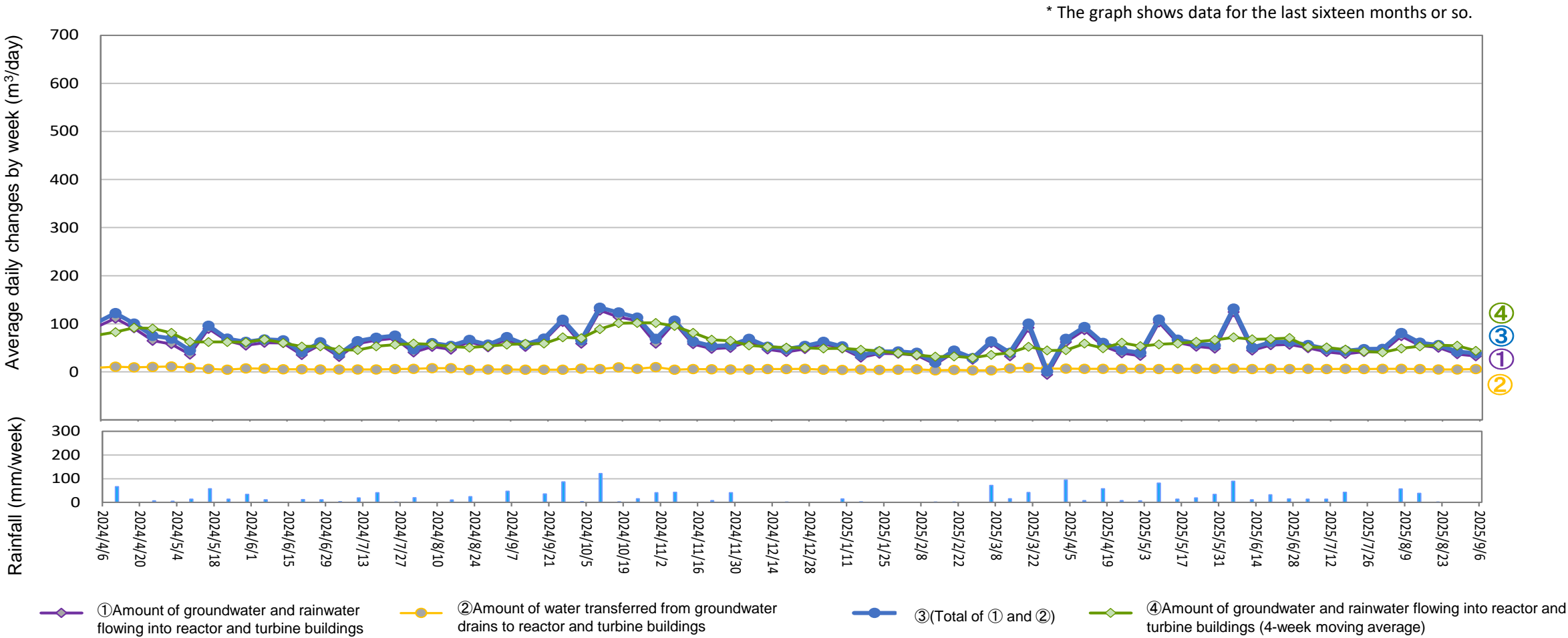
Amount of water transferred from groundwater drains to reactor and turbine buildings (From August 28, 2025 to September 3, 2025)
