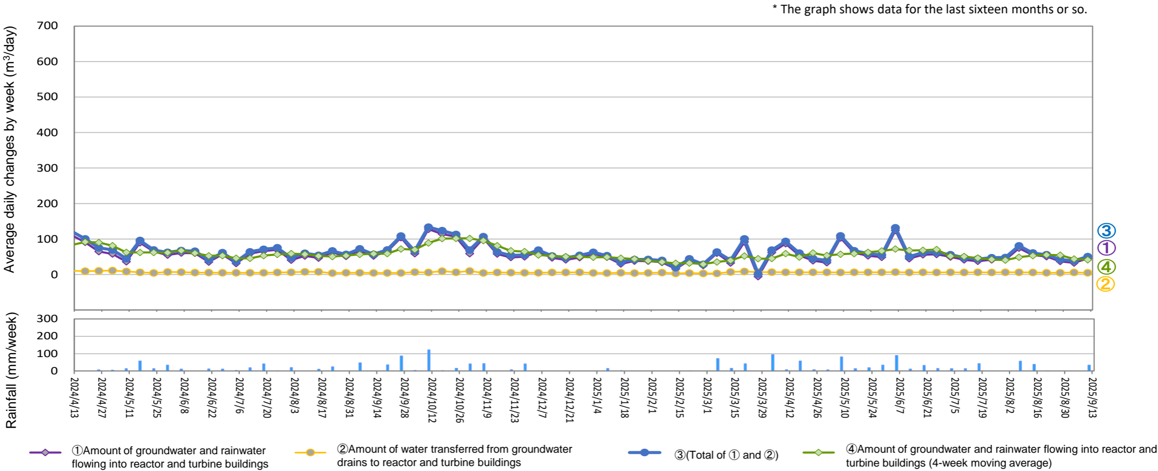
Amount of water transferred from groundwater drains to reactor and turbine buildings (From September 4, 2025 to September 10, 2025)
