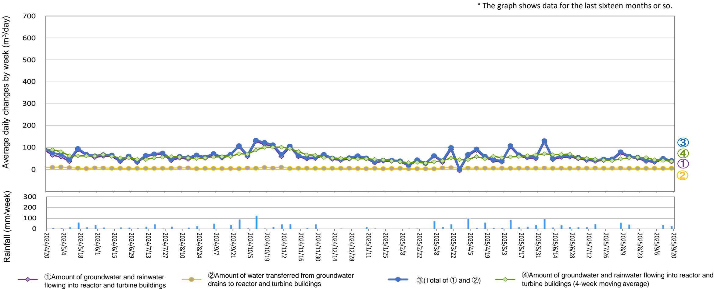
Amount of water transferred from groundwater drains to reactor and turbine buildings (From September 11, 2025 to September 17, 2025)
