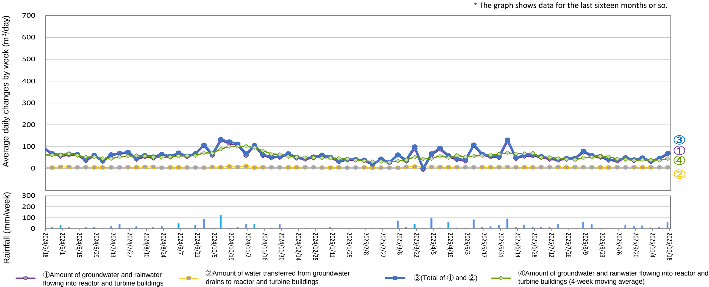
Amount of water transferred from groundwater drains to reactor and turbine buildings (From October 9, 2025 to October 15, 2025)
