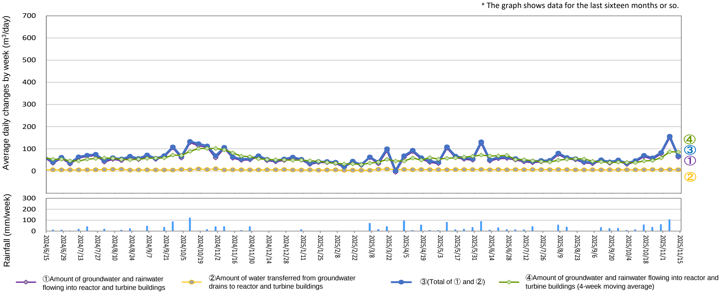
Amount of water transferred from groundwater drains to reactor and turbine buildings (From November 6, 2025 to November 12, 2025)
