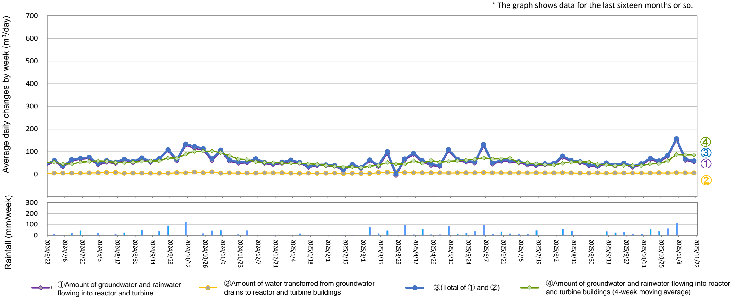
Amount of water transferred from groundwater drains to reactor and turbine buildings (From November 13, 2025 to November 19, 2025)
