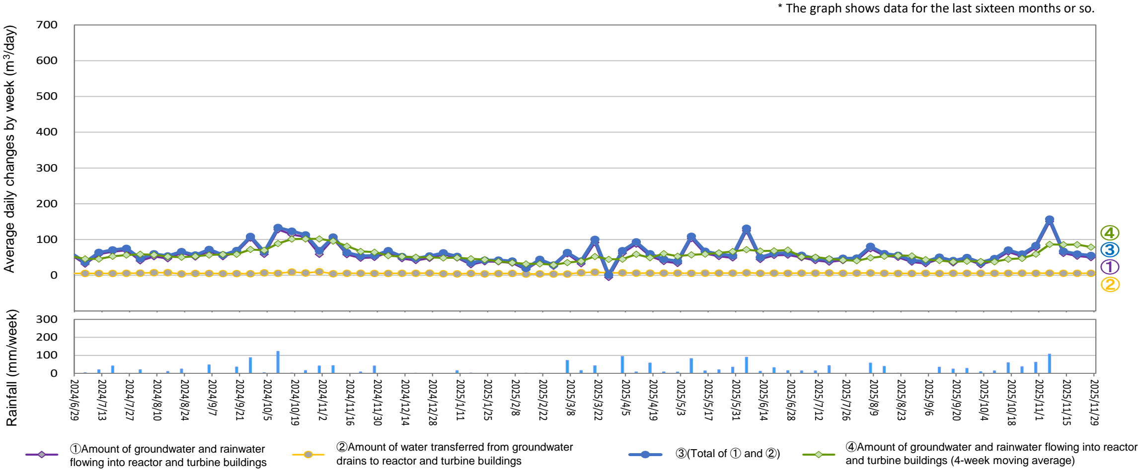
Amount of water transferred from groundwater drains to reactor and turbine buildings (From November 20, 2025 to November 26, 2025)
