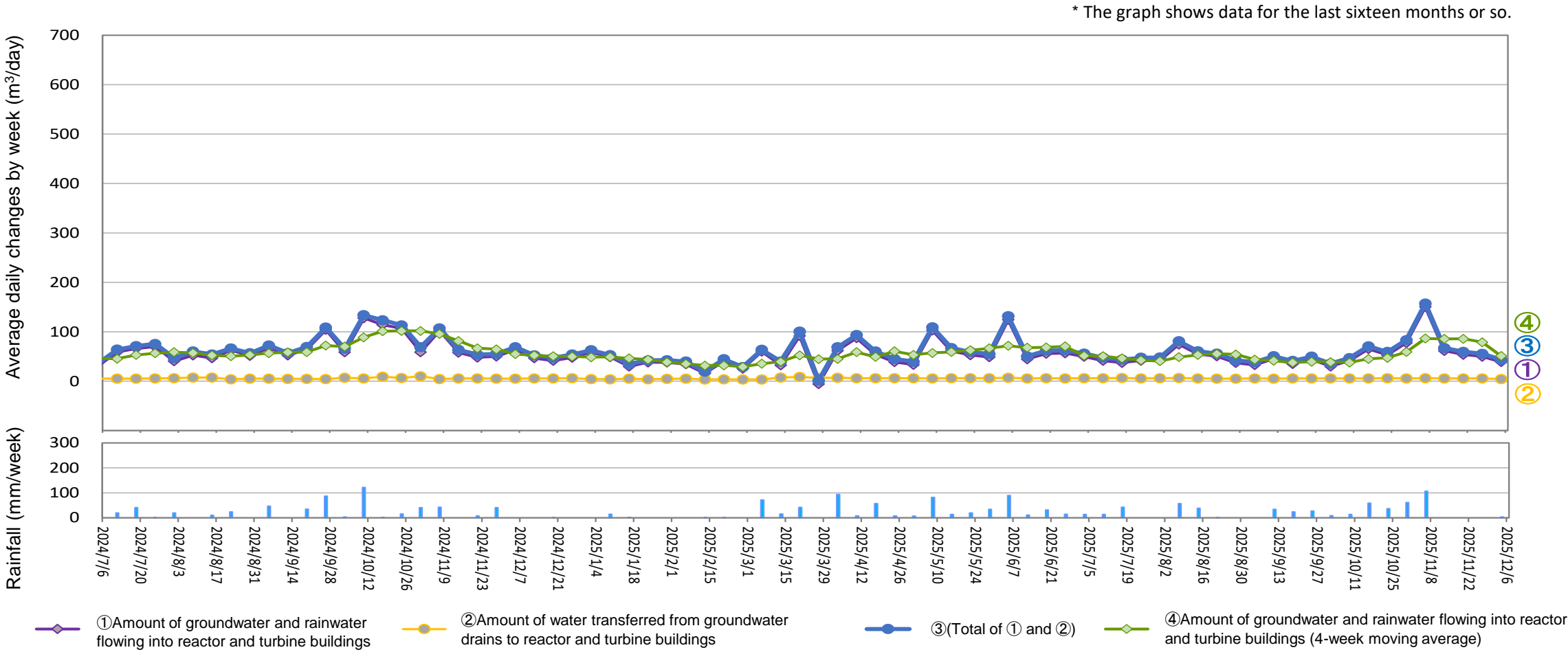
Amount of water transferred from groundwater drains to reactor and turbine buildings (From November 27, 2025 to December 3, 2025)
