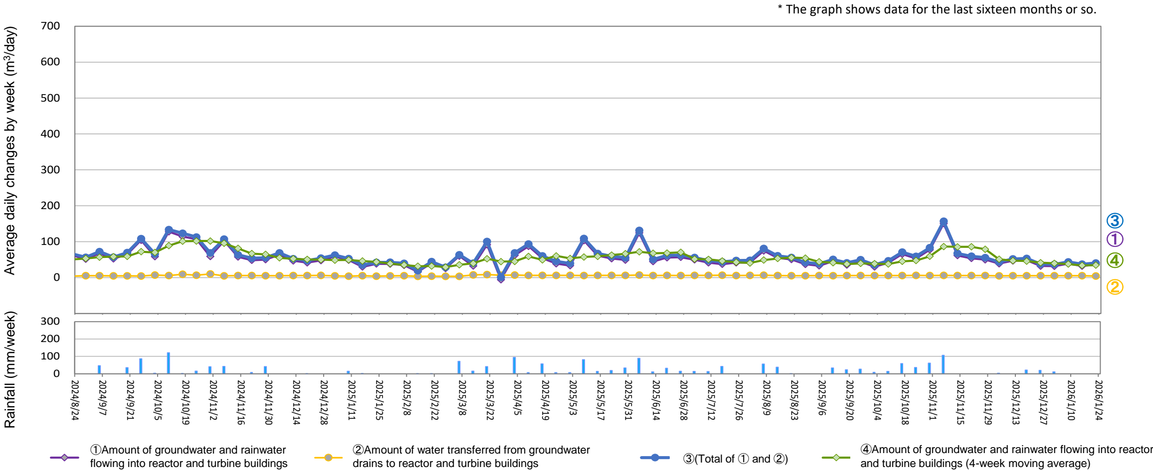
Amount of water transferred from groundwater drains to reactor and turbine buildings (From January 15, 2026 to January 21, 2026)
