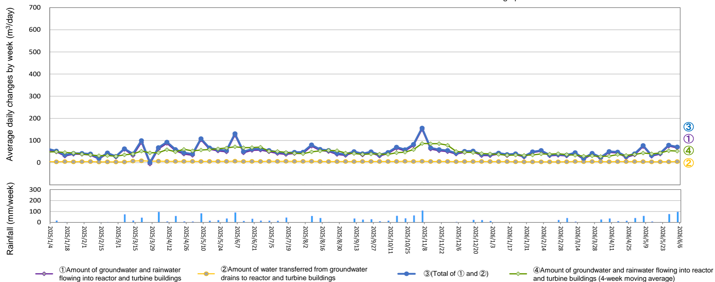
Amount of water transferred from groundwater drains to reactor and turbine buildings (From May 28, 2026 to June 3, 2026)
