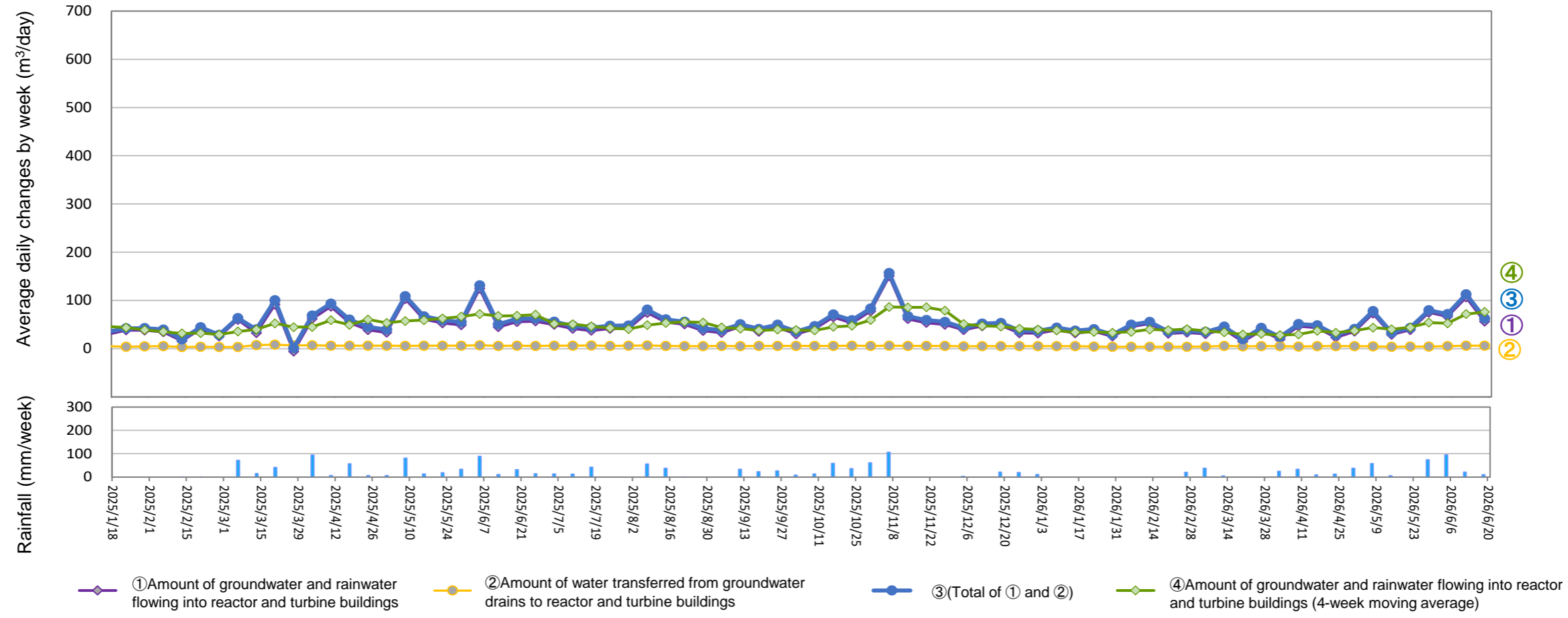
Amount of water transferred from groundwater drains to reactor and turbine buildings (From June 11, 2026 to June 17, 2026)
