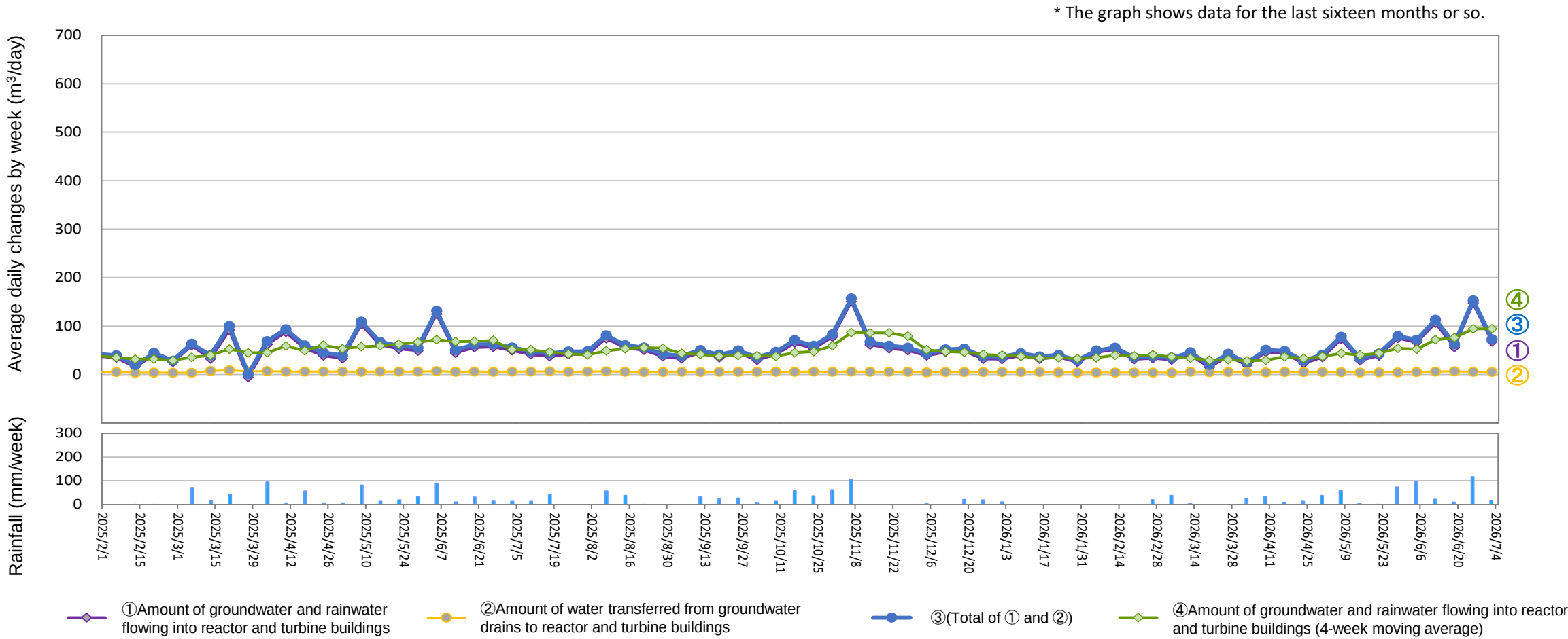
Amount of water transferred from groundwater drains to reactor and turbine buildings (From June 25, 2026 to July 1, 2026)
