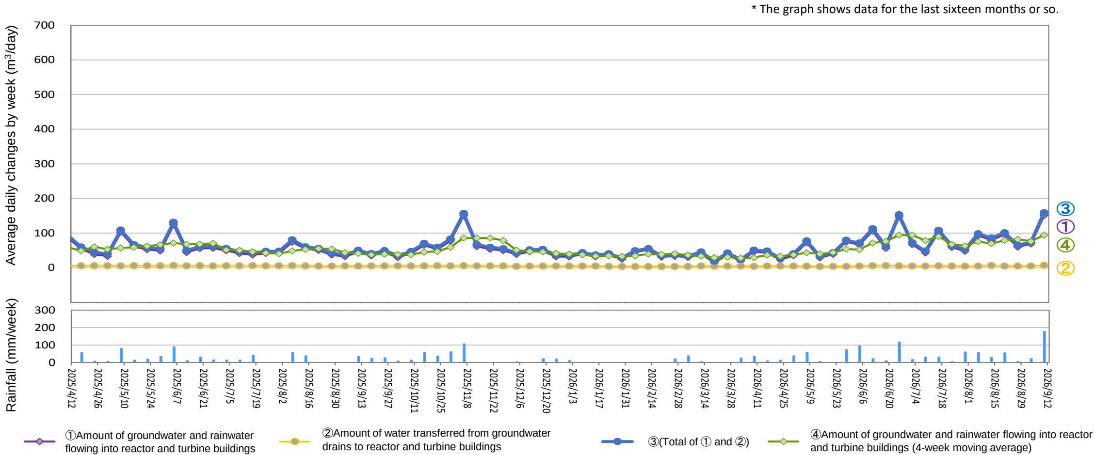
Amount of water transferred from groundwater drains to reactor and turbine buildings (From September 3, 2026 to September 9, 2026)
