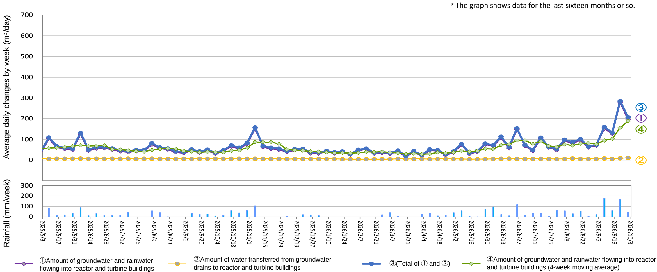
Amount of water transferred from groundwater drains to reactor and turbine buildings (From September 24, 2026 to September 30, 2026)
