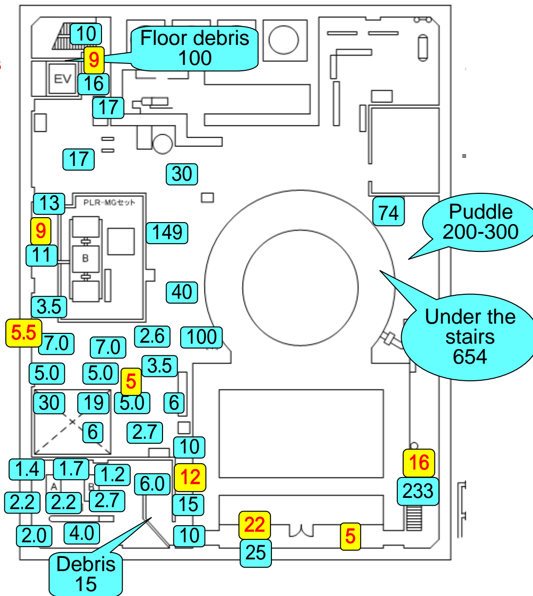
Unit 1 Reactor Building 3F
