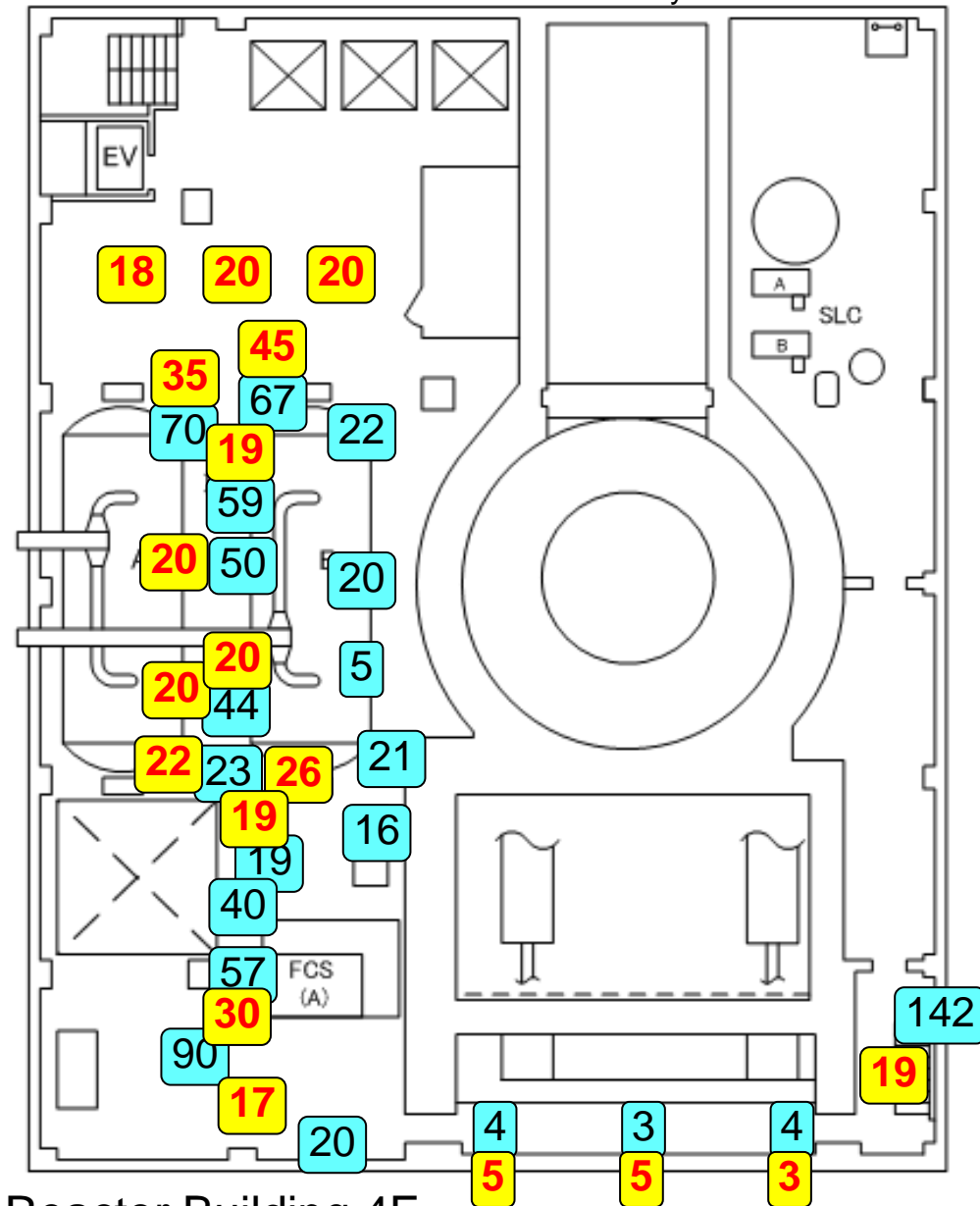
Unit 1 Reactor Building 4F
